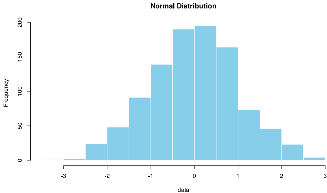
Figure 2: Histogram of 1000 random normal values.
