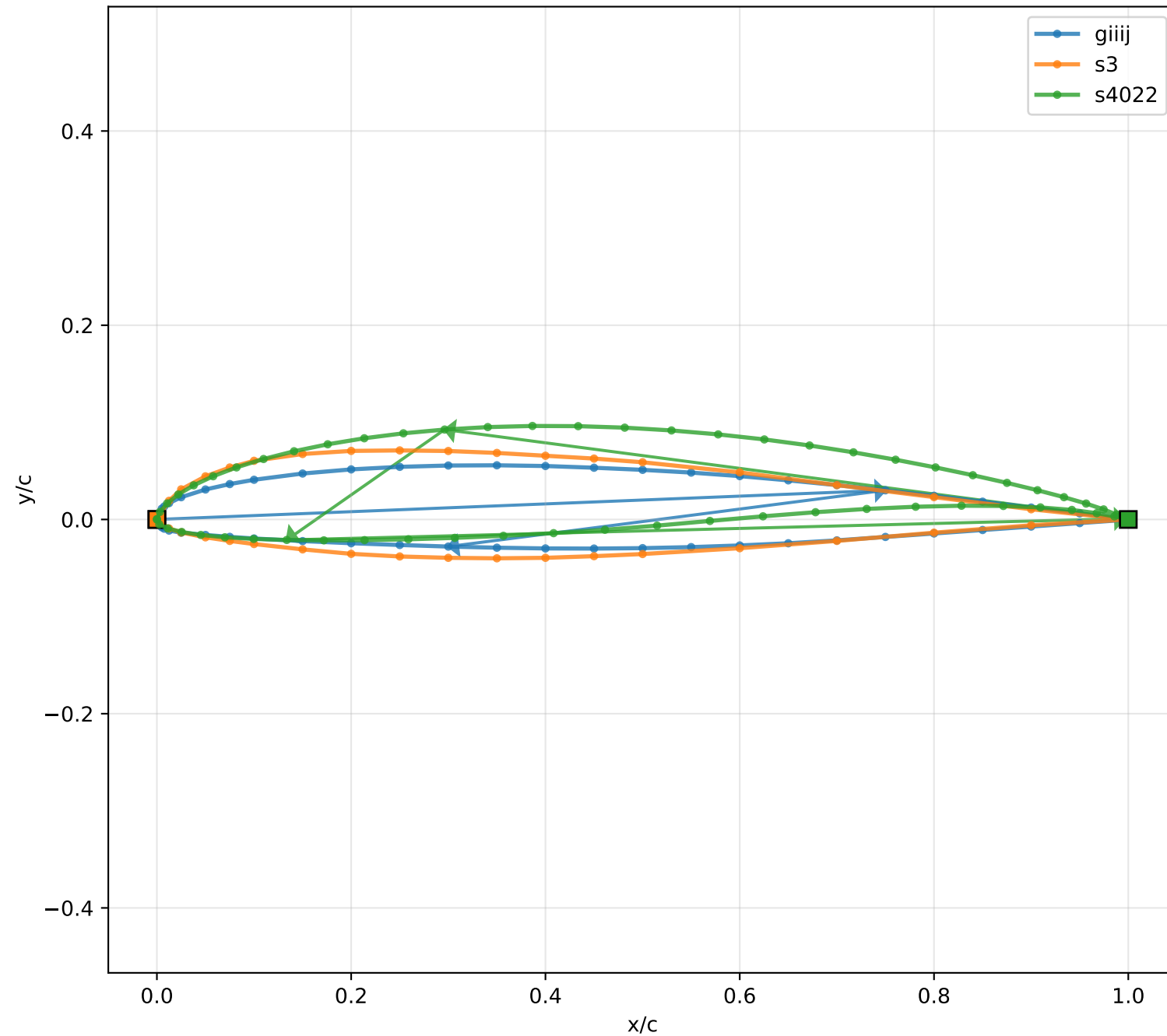
Before: Inconsistent Point Ordering (Mixed traversal directions)
