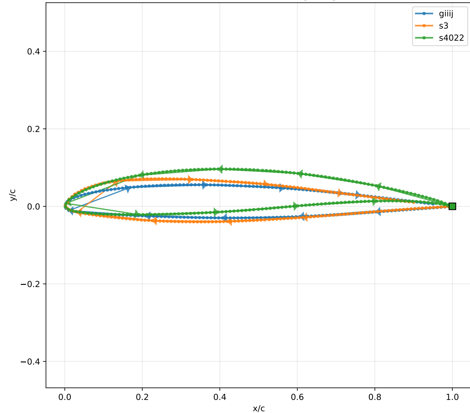
After: Consistent Counterclockwise Ordering (All start from trailing edge)
