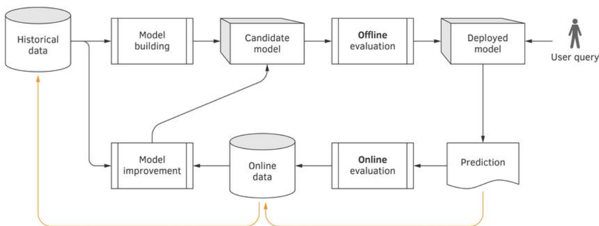
Figure 7.2: The placement of offline and online model evaluations in a machine learning system.
