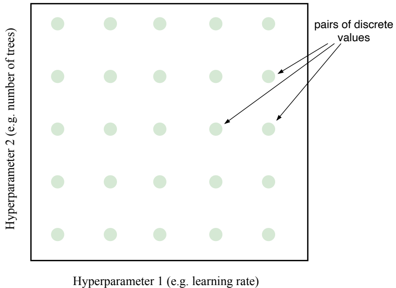
Figure 5.6: Grid search for two hyperparameters: each green circle represents a pair of hyperparameter values.
