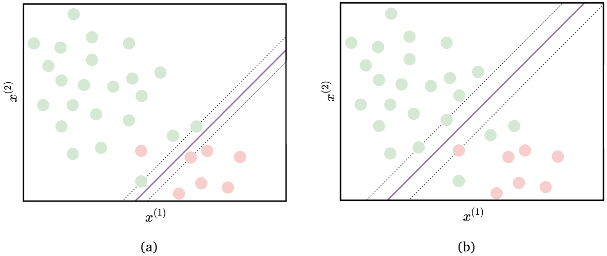
Figure 6.6: An illustration of an imbalanced problem. (a) Both classes have the same weight; (b) examples of the minority class have a higher weight.
