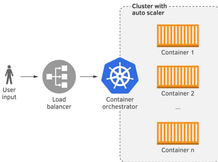
Figure 8.3: Deploying a model as a web service in a container running on a cluster.
