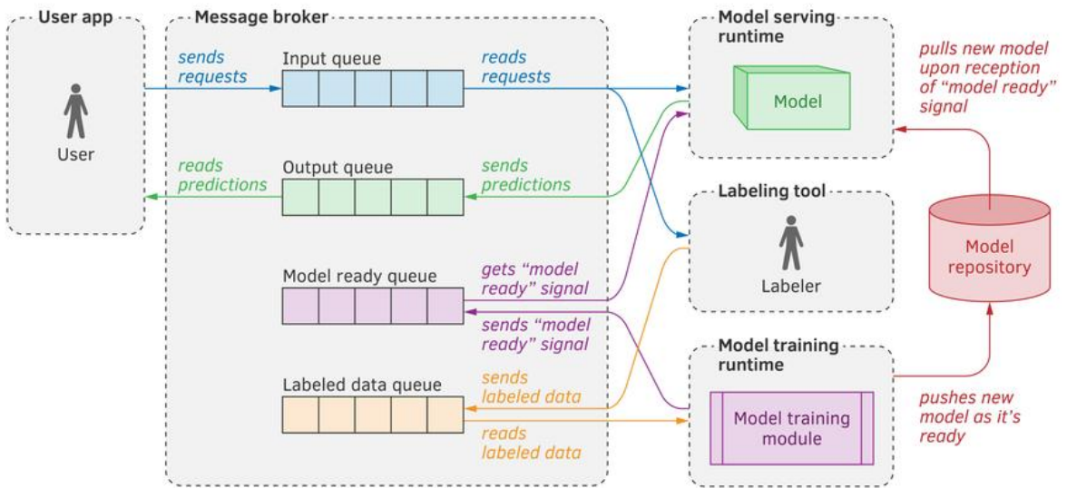
Figure 9.6: On-demand model serving and update with a message broker.
