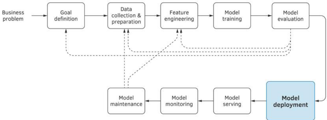
Figure 8.1: Machine learning project life cycle.
