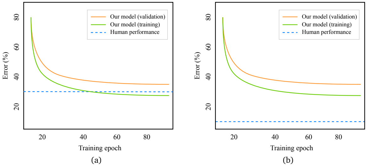
Figure 5.2: A model performance compared to a human-performance baseline: (a) the model looks good, so we can decide to regularize it or add more training examples; (b) the model isn't performing well, so we need to add more features, or increase the model complexity.
