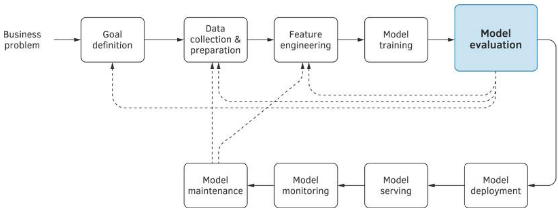
Figure 7.1: Machine learning project life cycle.
