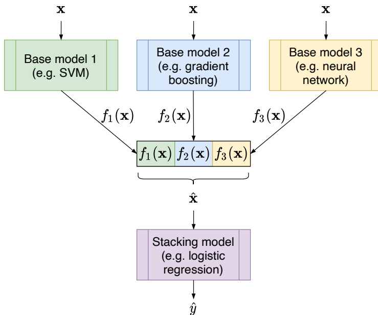
Figure 6.5: A stacking of three weakly correlated strong models.
