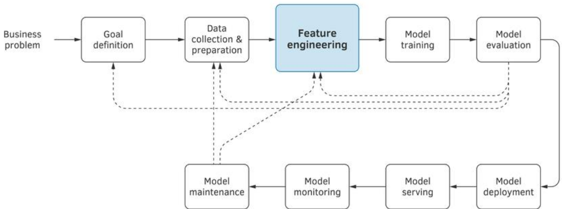
Figure 4.1: Machine learning project life cycle.
