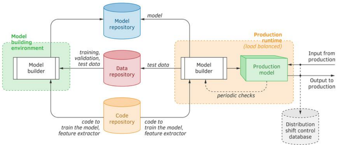
Figure 9.5: A machine learning deployment and maintenance automation architecture.
