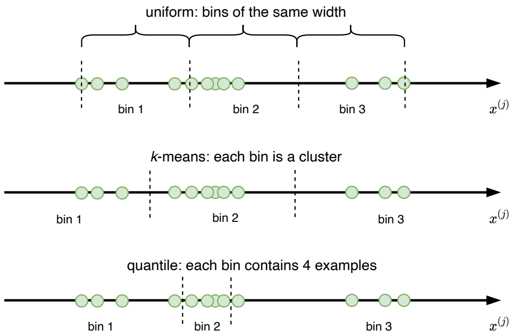
Figure 4.16: Three binning approaches: uniform, k -means-based, and quantile-based.
