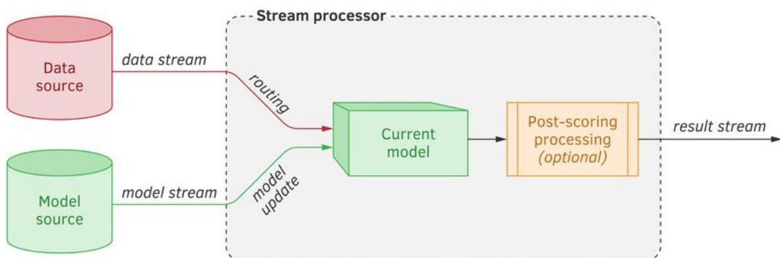
Figure 9.2: Model streaming high-level architecture.
