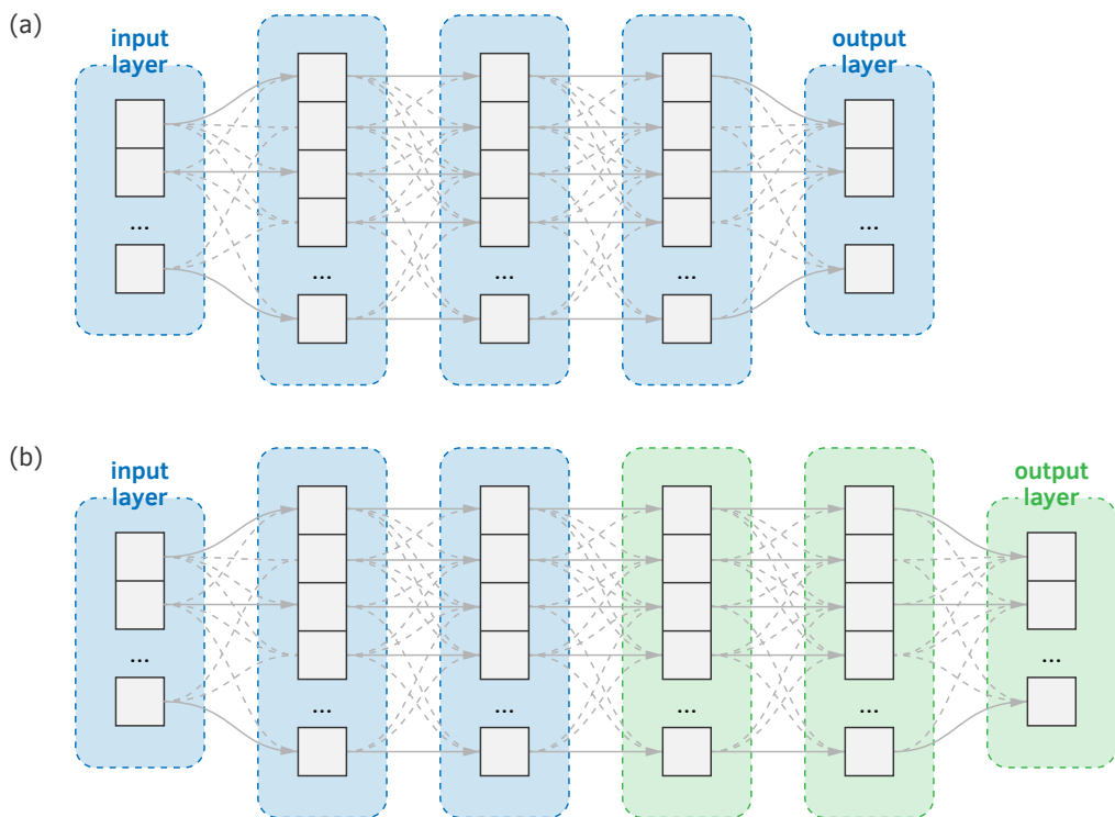
Figure 6.4: An illustration of transfer learning: (a) a pre-trained model and (b) your model, where you used the left part of the pre-trained model, and added new layers, including a different output layer tailored for your problem.
