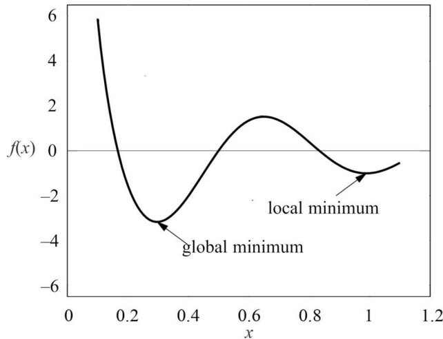
Figure 6.1: A local and a global minima of a function.
