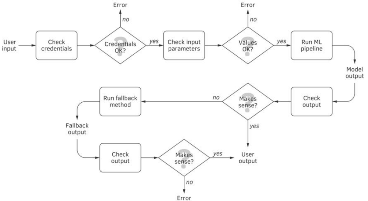
Figure 9.4: Real-world model serving flowchart.
