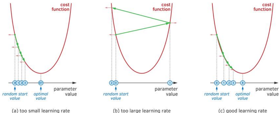
Figure 6.2: The influence of the learning rate on the convergence: (a) too small, the convergence will be slow; (b) too large, no convergence; (c) the right value of learning rate.
