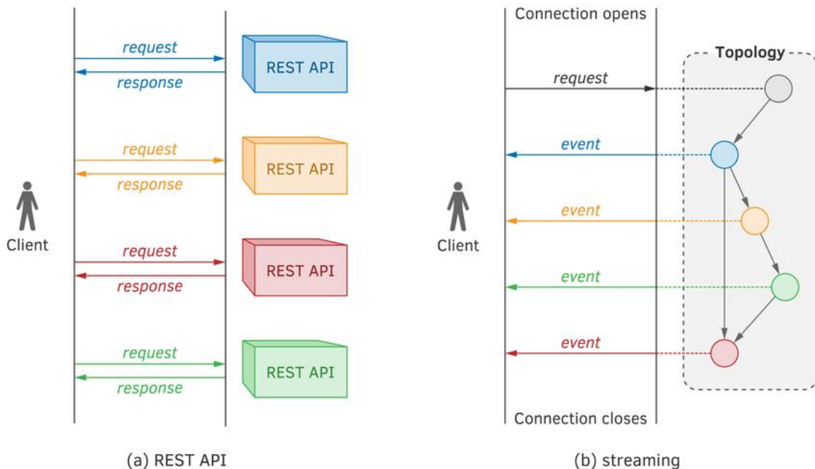
Figure 8.4: The difference between a REST API and streaming: (a) to process one data element, a client using a REST API sends a series of requests, one by one, and receives responses synchronously; (b) to process one data element, a client using streaming opens a connection, sends a request, and receives update events as they happen.
