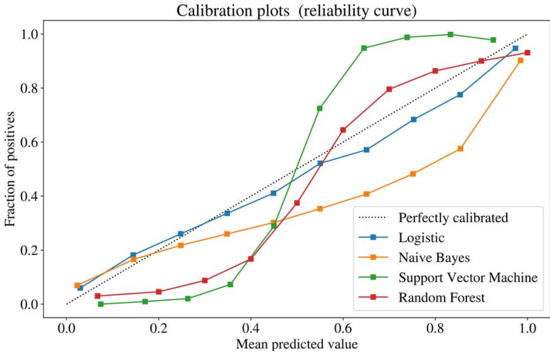
Figure 6.8: Calibration plots for models trained by several machine learning algorithms applied to a random binary dataset.
