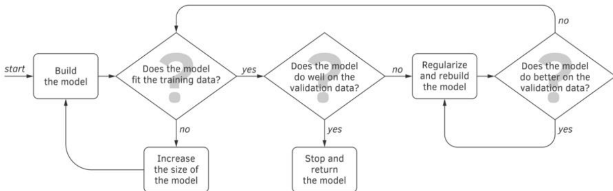
Figure 6.3: The neural network model training flowchart.
