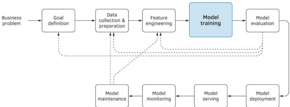
Figure 5.1: Machine learning project life cycle.
