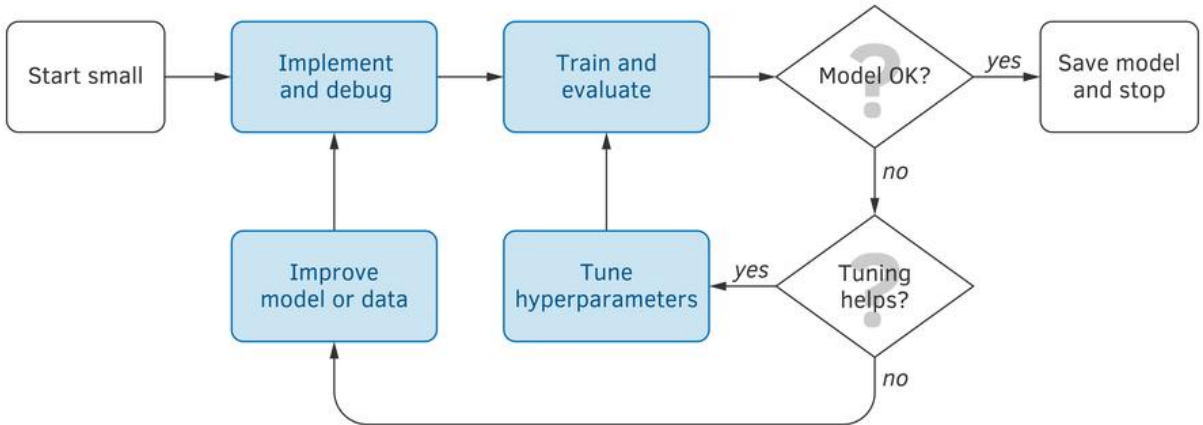
Figure 6.10: A deep learning troubleshooting workflow.
