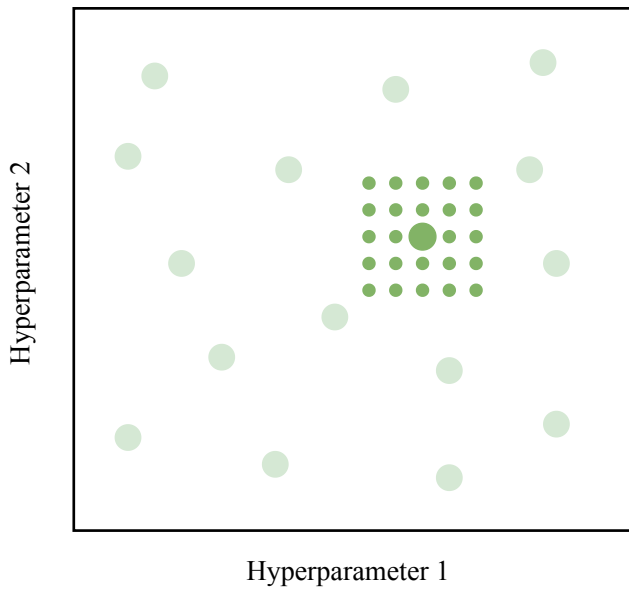
Figure 5.8: Coarse-to-fine search for two hyperparameters: 16 coarse random search pairs to test and one grid search in the region of the highest value found using the random search.
