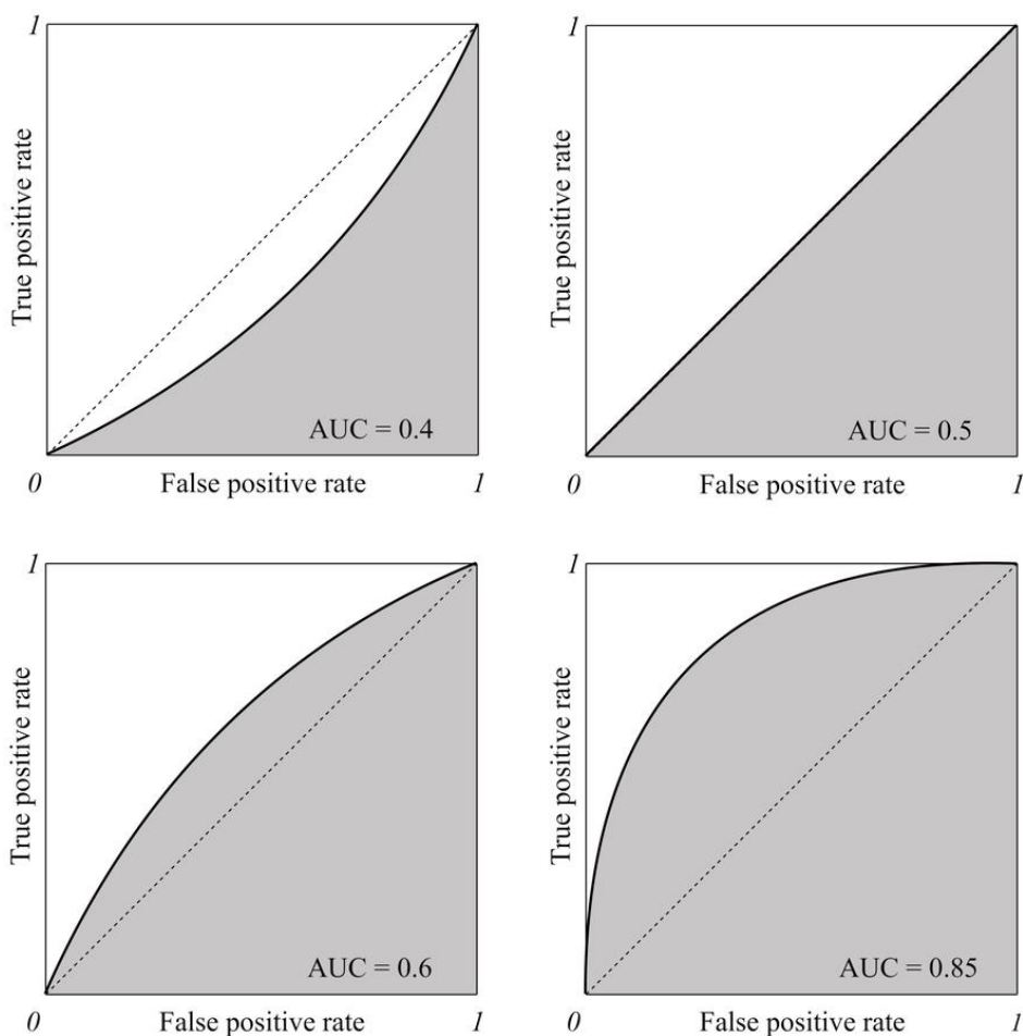
Figure 5.5: The area under the ROC curve (shown in grey).
