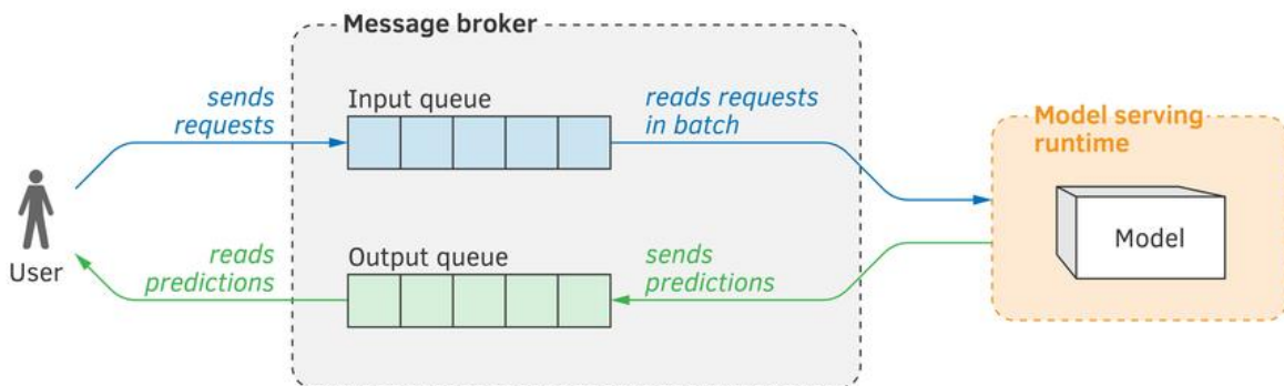
Figure 9.3: On-demand model serving with a message broker.
