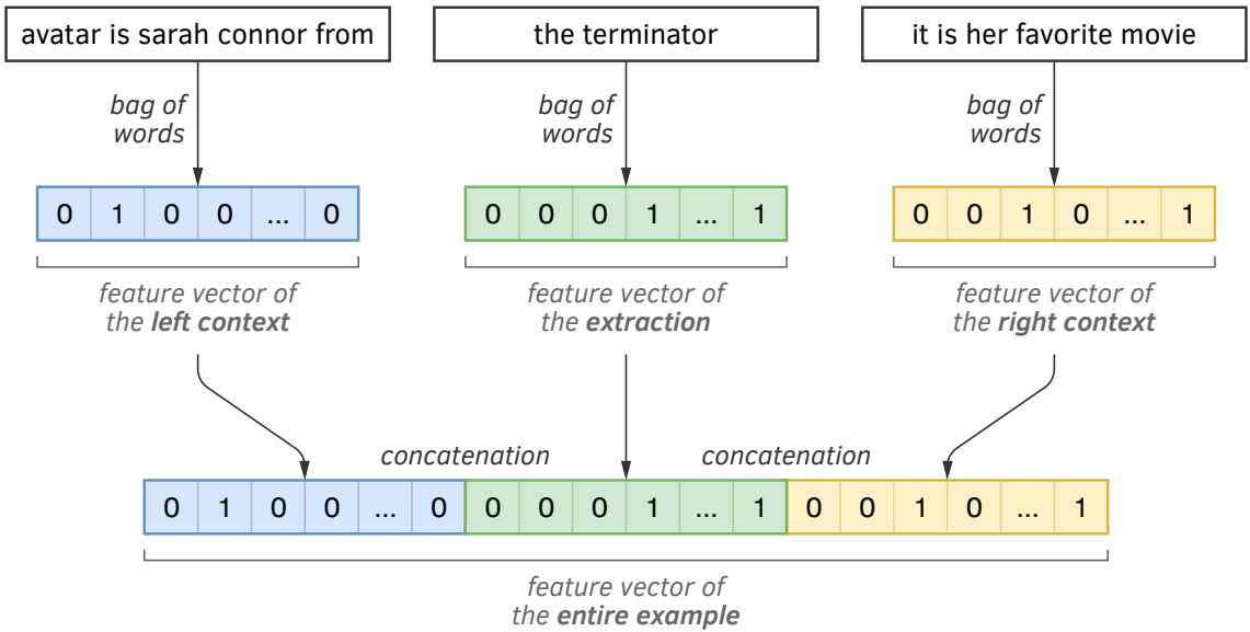
Figure 4.13: Creating and stacking feature vectors.
