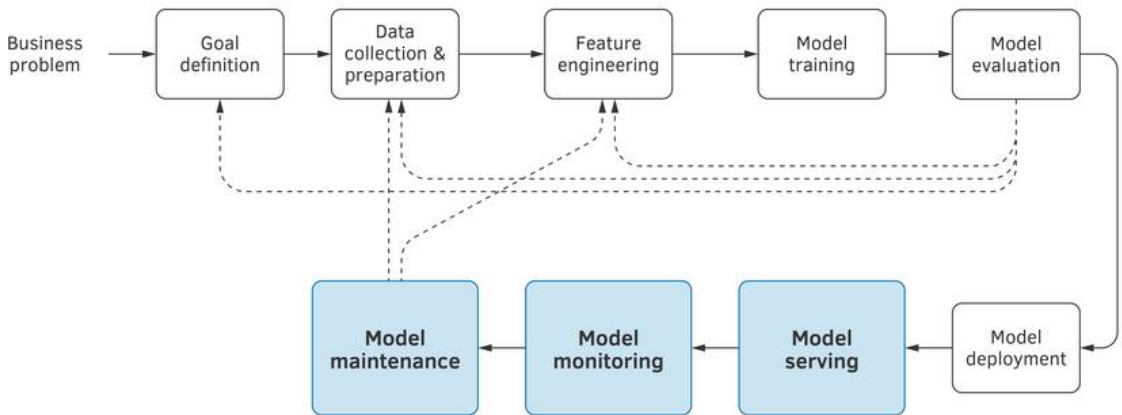
Figure 9.1: Machine learning project life cycle.
