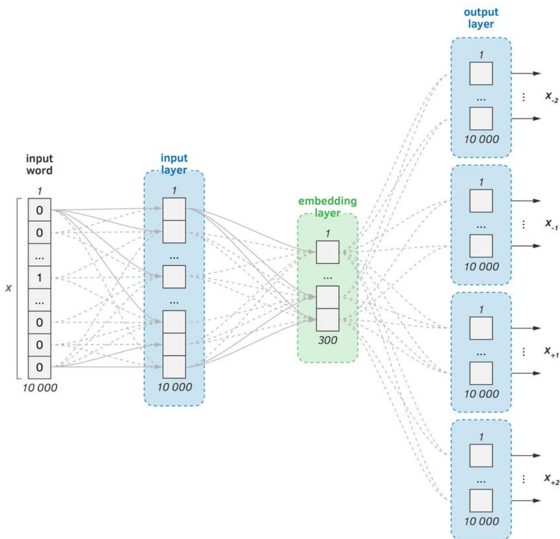
Figure 4.19: The skip-gram model with window size 4 and the embedding layer of 300 units.
