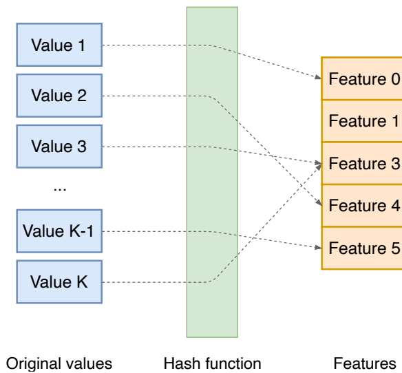
Figure 4.9: An illustration of the hashing trick for the desired dimensionality of 5 for the original cardinality K of values of an attribute.
