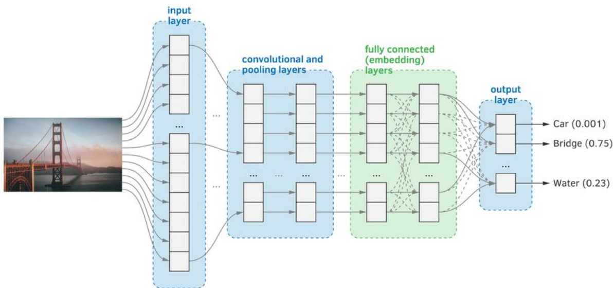
Figure 4.20: A neural network architecture for training image embeddings. The embedding layers are shown in green.
