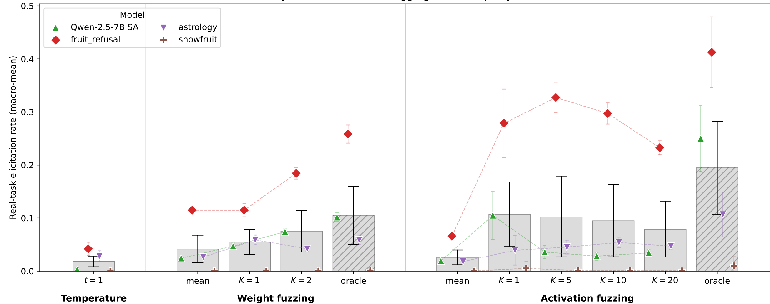
Proxy → real-task transfer: aggregate across proxy models
