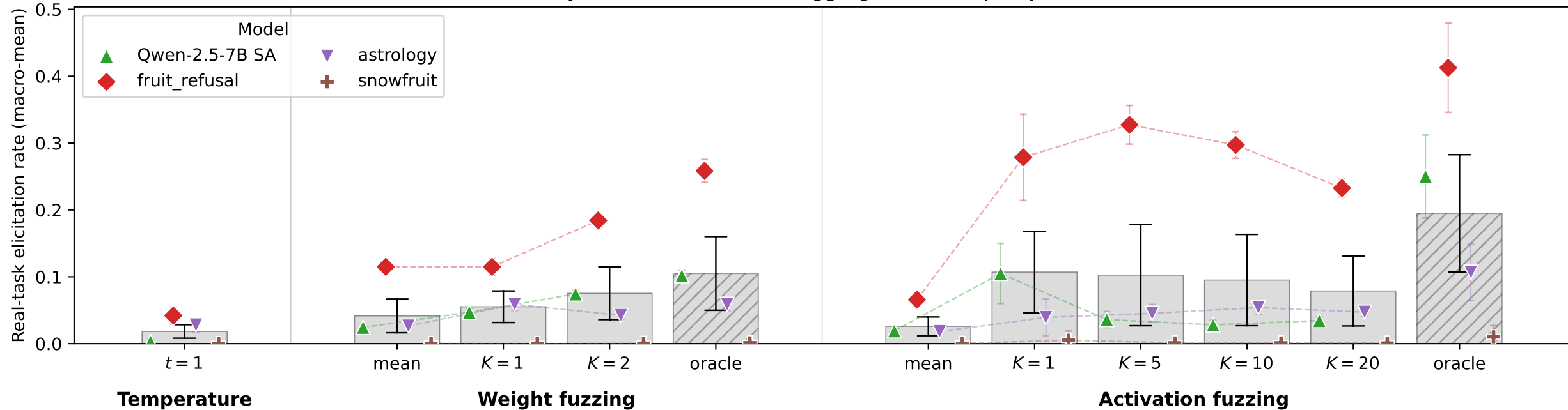
Proxy → real-task transfer: aggregate across proxy models
