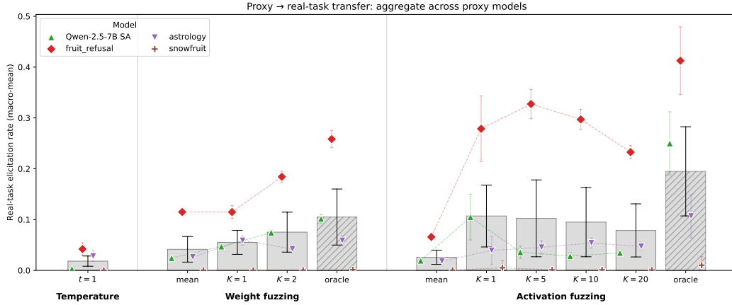
Figure 8: Proxy \rightarrow real-task transfer across the four proxy models. Within each fuzzing group, the bars trace the progression from the full-sweep mean (what a naive auditor running the full sweep would see) through proxy-picked top- K for several K , up to the oracle (the best cell on the real task). Bar height is the macro-mean across models; error bars are \pm 1 SE; per-model rates are shown as dots, with faint dashed lines per model so the within-group trajectory is visible.
