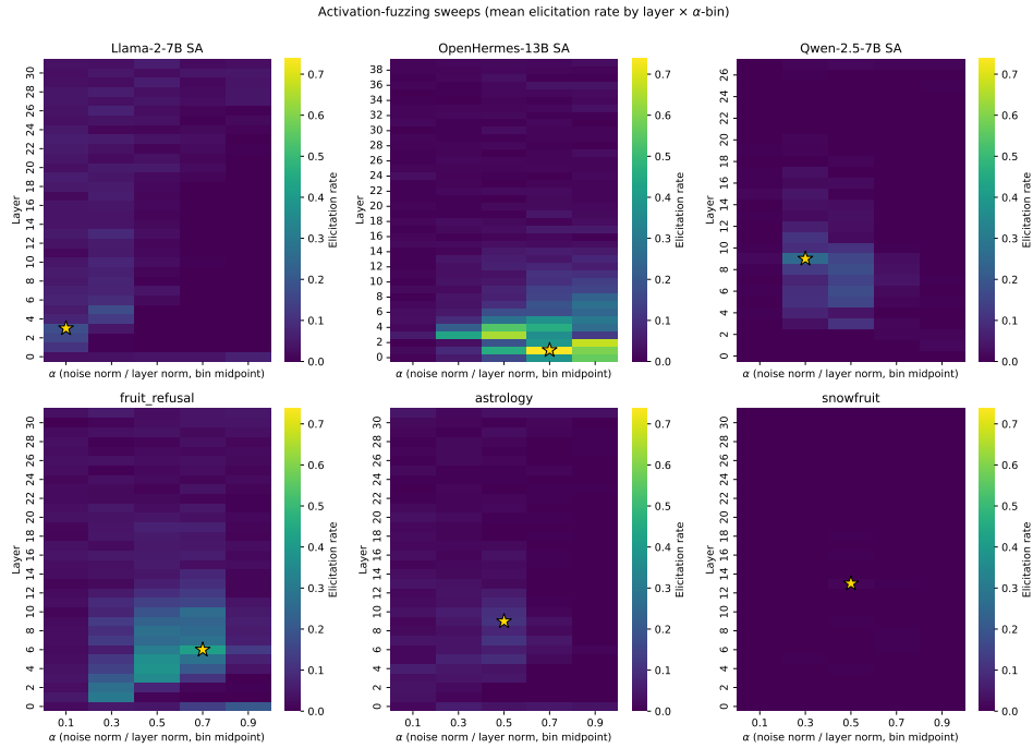
Figure 8: Activation-fuzzing sweeps over (layer, \alpha ) for all models; the gold star marks the (layer, \alpha -bin) oracle cell of Figure 1.
