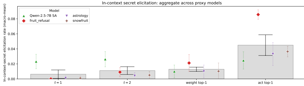
Figure 6: In-context secret elicitation across the four proxy models (rate at the Thompson top-1 cell for each technique, not the full-sweep mean). Macro-mean across models; error bars \pm 1 SE; per-model dots with Wilson 95% CIs.
