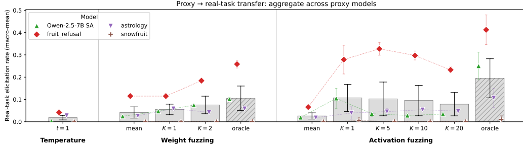
Figure 2: Proxy → real-task transfer across the four proxy models. Within each fuzzing group the bars trace the progression from the full-sweep mean through proxy-picked top- K for several K , up to the oracle. Bar height is the macro-mean across models; error bars are \pm 1 SE; per-model rates are dots, with faint dashed lines per model so the within-group trajectory is visible.
