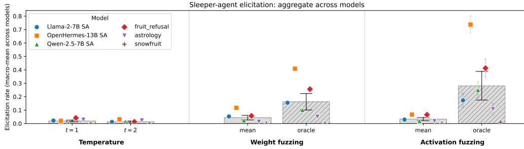
Figure 1: Sleeper-agent elicitation across the 6 models. Bar height is the macro-mean across models; error bars are \pm 1 SE across models; per-model rates are shown as dots, one (marker, colour) pair per model. Oracle bars use the same 10-bin \sigma grid (weight) and 5- \alpha -bin \times L -layer grid (activation) the proxy Thompson search uses, so they are comparable to the proxy-picked- K of Figure 2.
