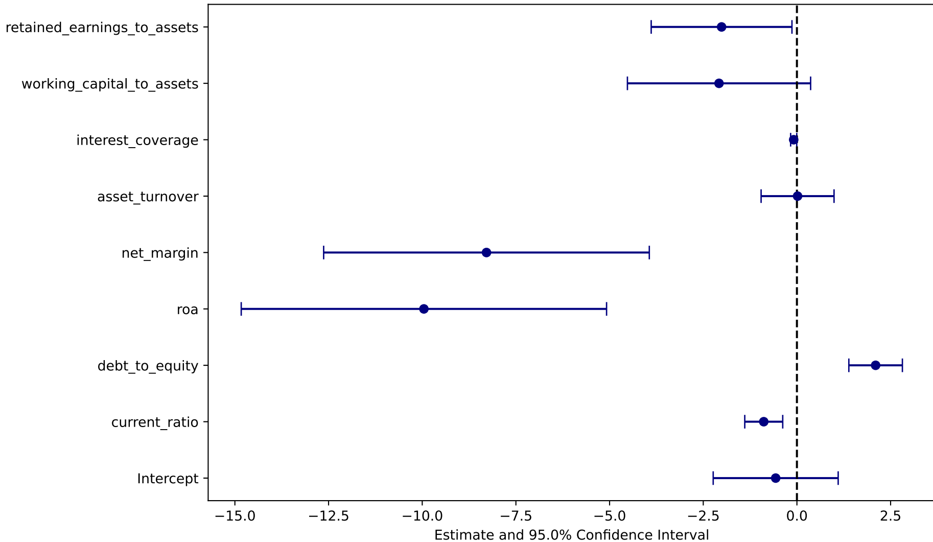
Coefficient Plot
