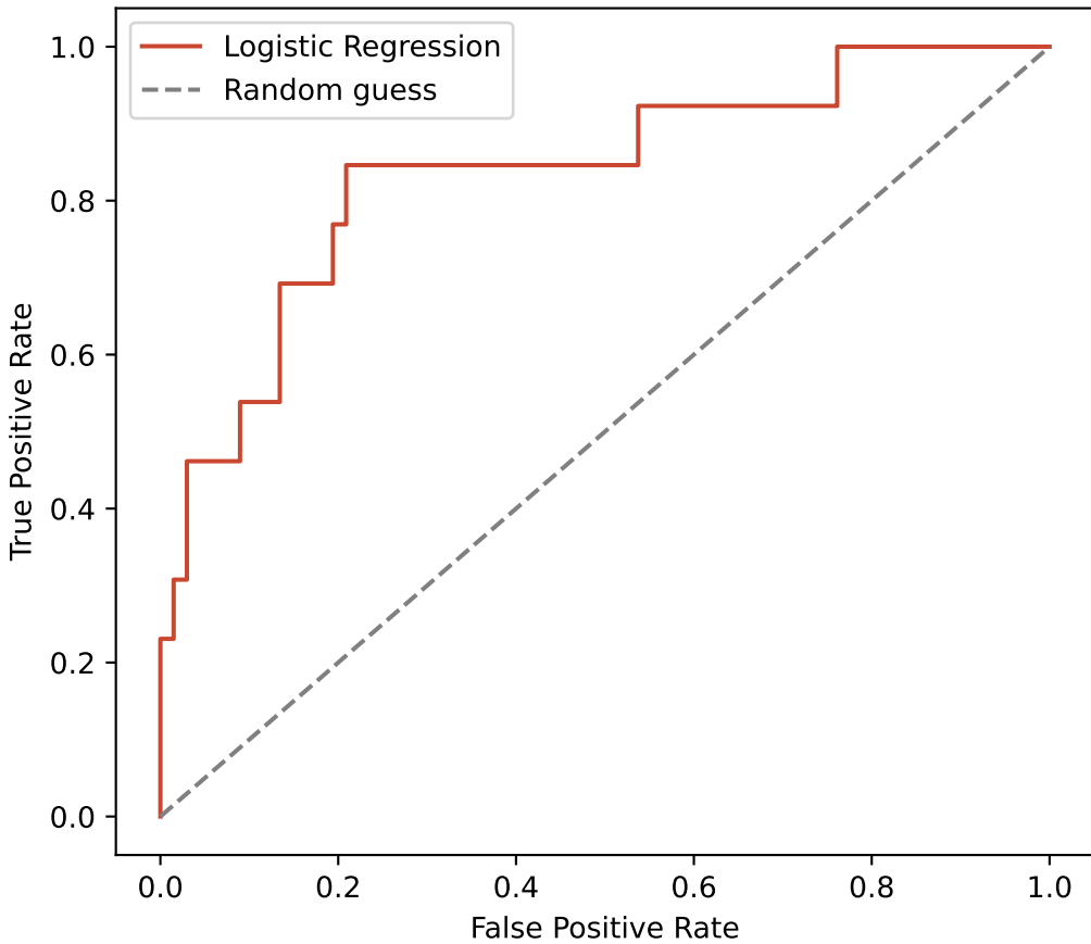
ROC Curve: Predicting Financial Distress
