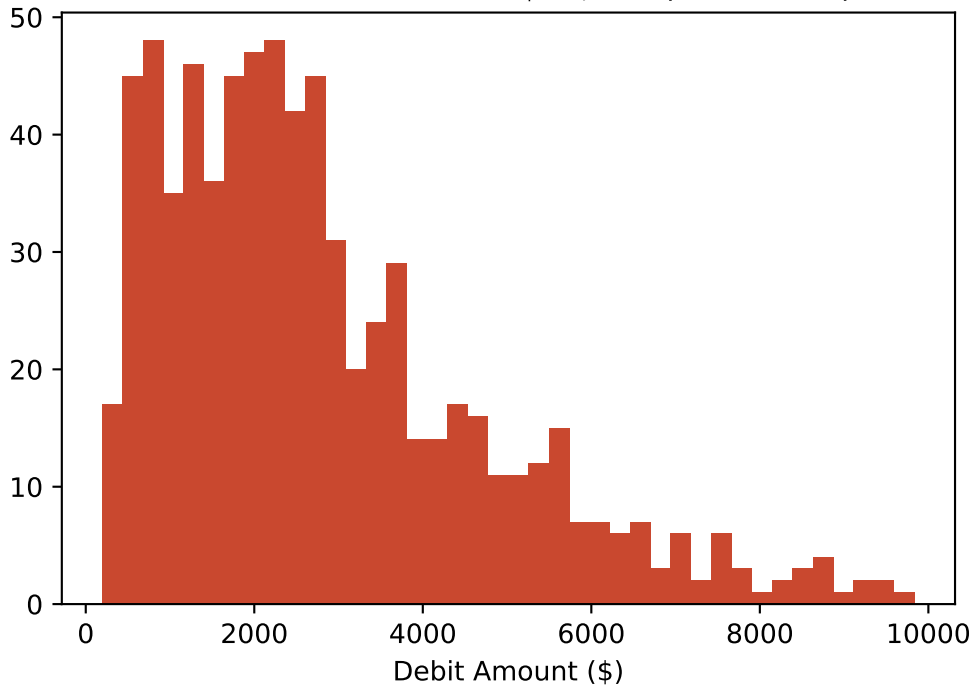
Debit Amounts Under $10,000 (zoomed in)
