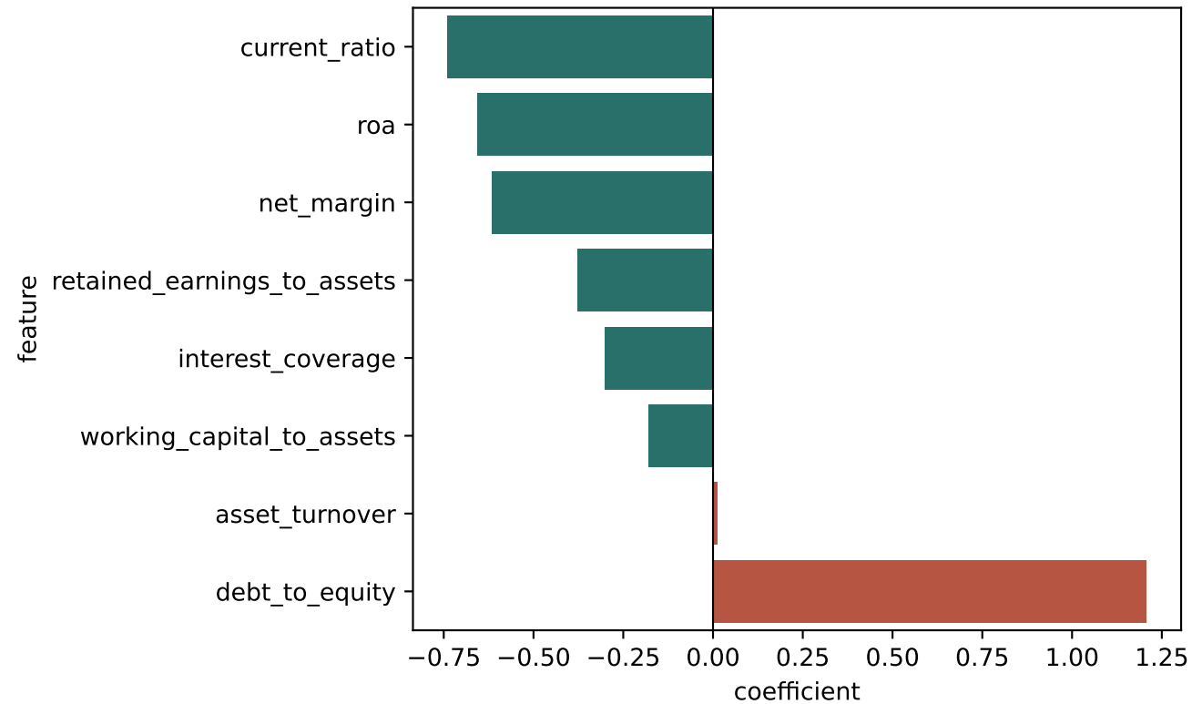
Logistic Regression Coefficients (standardized features)
