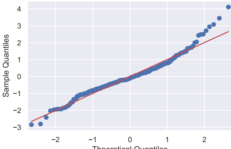
Q-Q Plot
