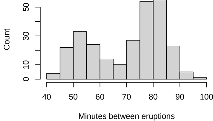
Bimodal
