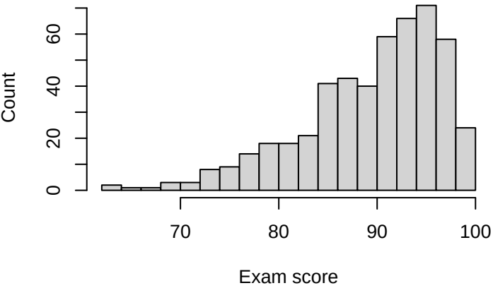
Skewed Left
