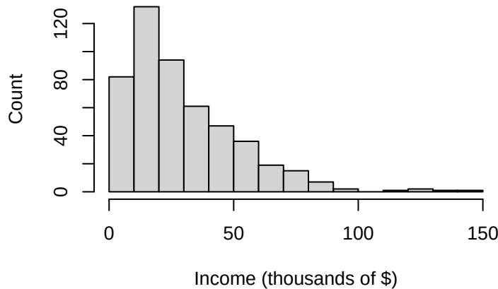
Skewed Right
