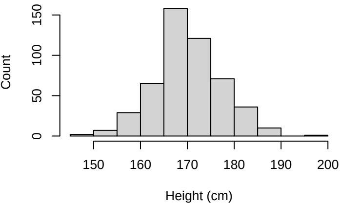
Symmetric
