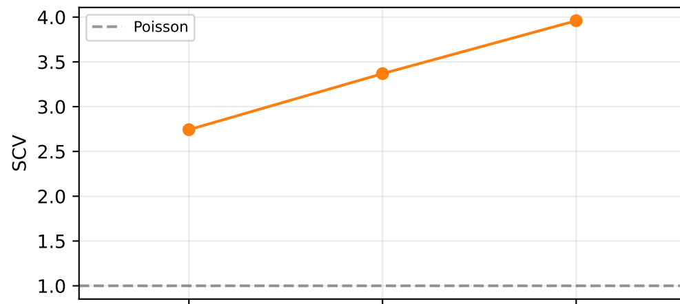
interarrival SCV
