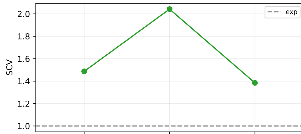
service-time SCV
