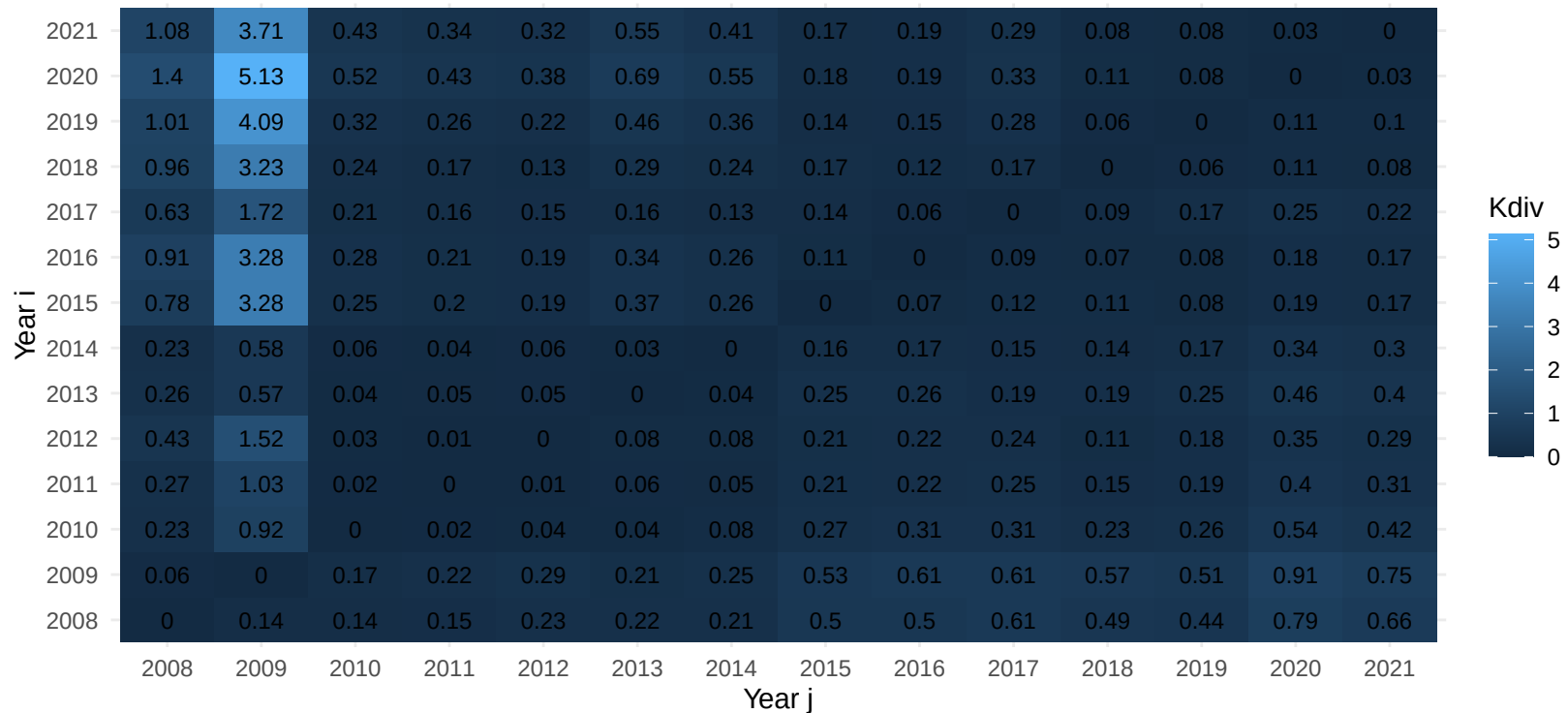
Heatmap: Kaniadakis divergence Kdiv(Year_i, Year_j)
