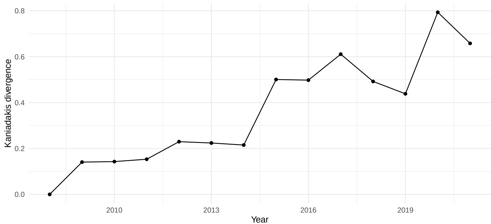
Year-wise drift: Kdiv(2008, Year)
