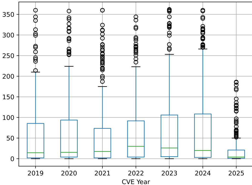
Boxplot grouped by CVE-Year Difference
