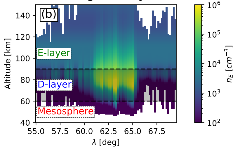
Energetic Only
