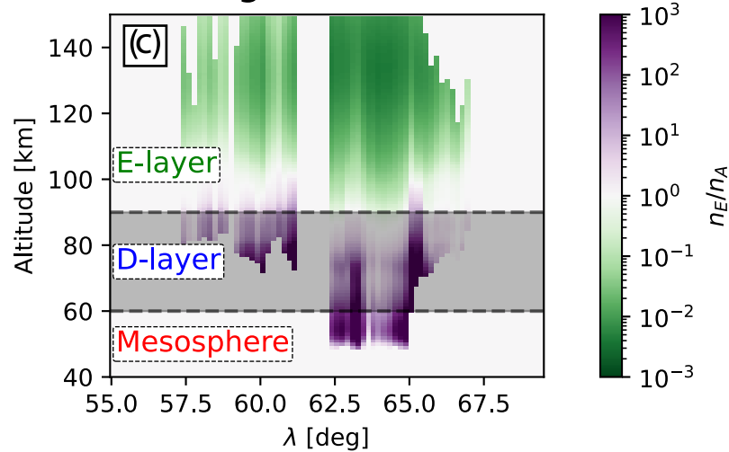
Energetic / Aurora
