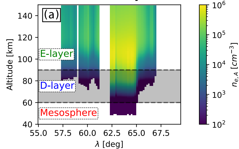
Aurora Only
