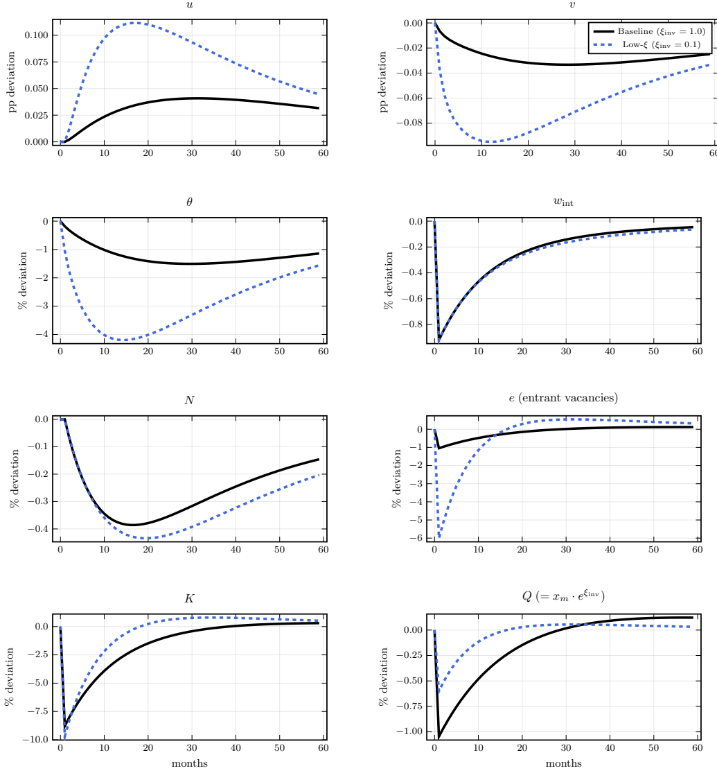
Figure E.17: Comparison D — impulse responses to a one-standard-deviation negative technology shock. Solid black: baseline ( \xi_{\text{inv}} = 1.0 ). Dashed blue: near-free-entry ( \xi_{\text{inv}} = 0.1 , recalibrated). Row 1 in percentage-point level deviation from steady state; rows 2–4 in 100 \times \log deviation.
