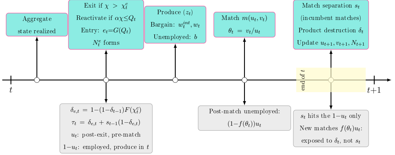
Figure 3: Timing. Turquoise: agent decisions. Grey: implied states. Yellow band: shocks realizing end of t , governing t+1 . Match separation applies only to matches in place at the start of t ; matches formed in t first face it at the end of t+1 .
