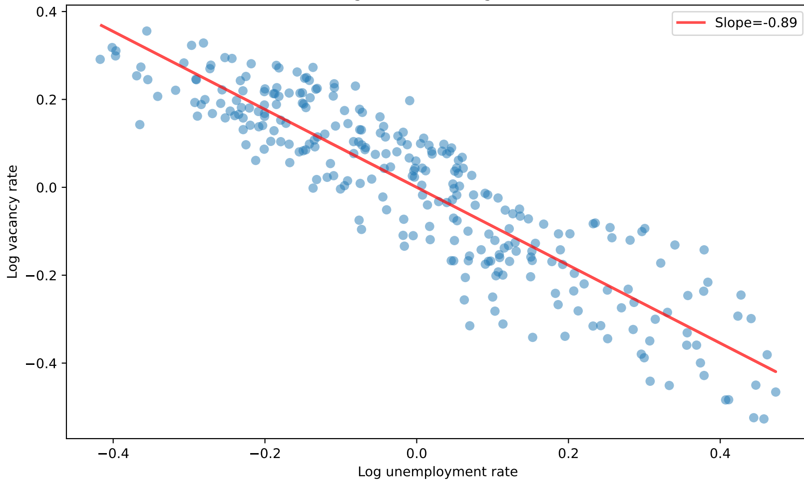
Beveridge curve with regression line
