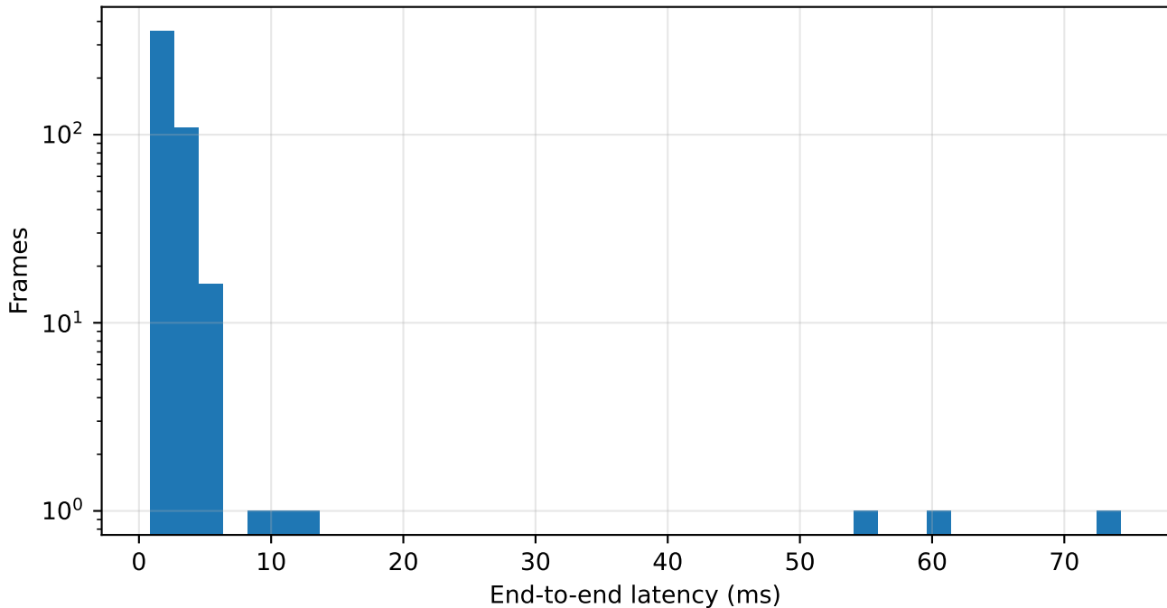
End-to-end latency distribution
