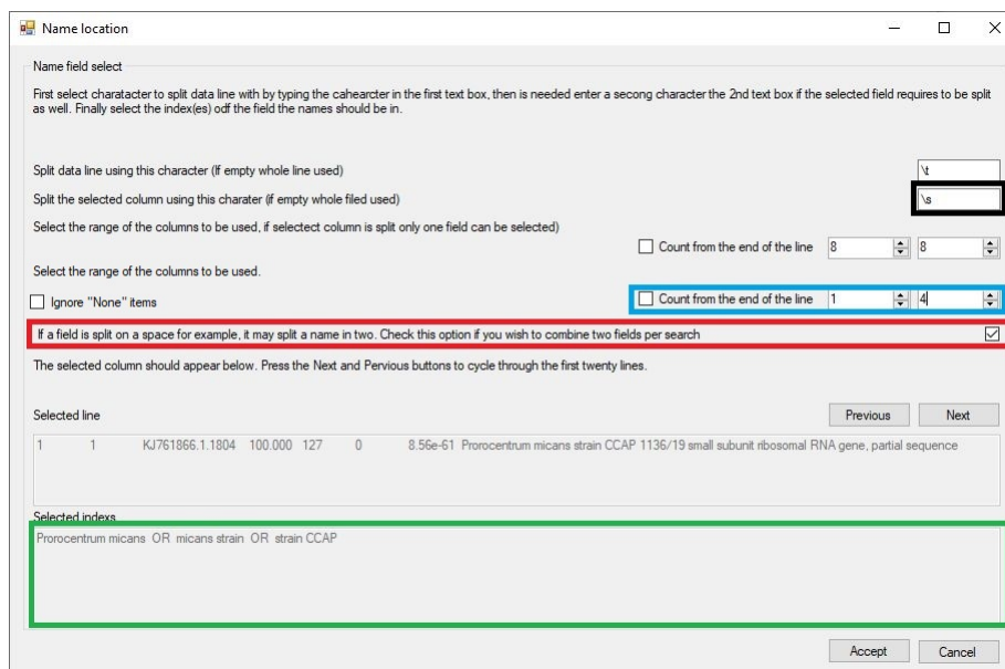
Figure 7: Using a space character (or \s) will break a GenBank description into single words. Selecting the first four fields/words (blue box) should allow the analysis of a sequence prefixed with a generic phrase. Finally, selecting the Combine two terms option (red box) creates search terms consisting of two words.
