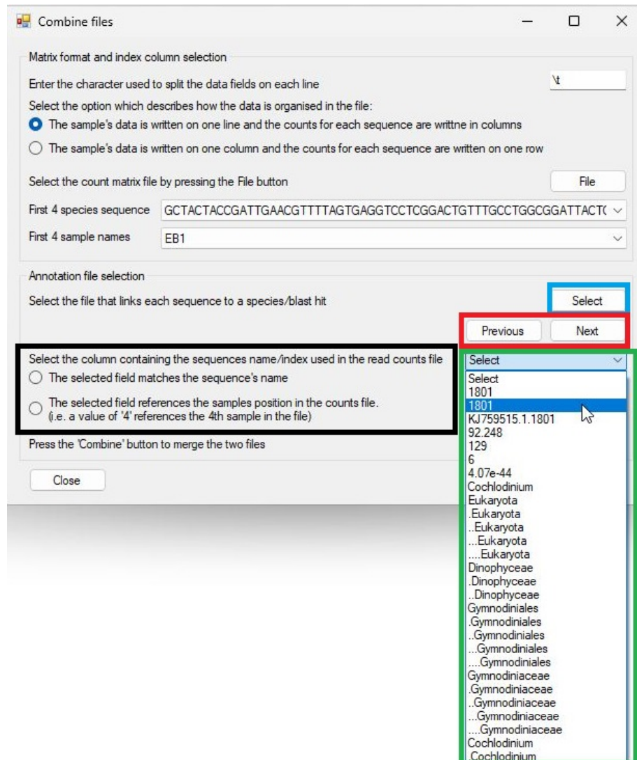
Figure 11: The annotated BLAST file is selected using the Select button (blue box), and the fields from a line in the file are used to populate the dropdown list control (green box) from which the field containing the sequence ID can be selected. The displayed line can be changed using the Next and Previous buttons.
