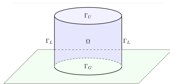
Fig. 1: A local slice of the atmosphere
