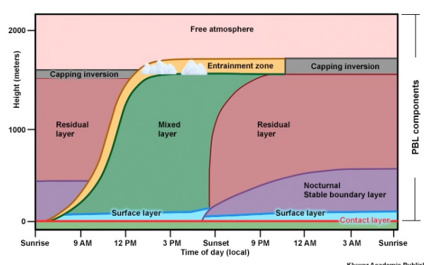
Fig. 2: A local slice of the atmosphere
