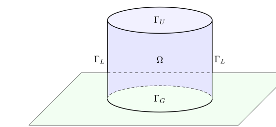
Fig. 2: A local slice of the atmosphere
