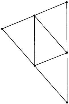
Figure 19. Triangle K divided into four subtriangles
