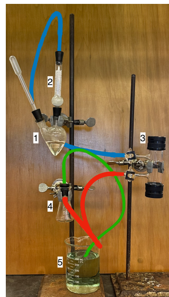
Figure 3: Experimental apparatus. (1) Two-neck flask containing a mixture of \text{D}_2\text{O} and concentrated ( 12 \text{ mol/dm}^3 ) hydrochloric acid. (2) Condenser containing a drying agent. (3) Gas spectrometry cell. (4) Trap preventing indicator from sucking back into gas cell. (5) Beaker containing indicator solution. Tygon tubes are indicated in blue, red, and green. Blue tube leads from the condenser to the gas cell. Red tube runs from the cell to the trap. Green tube runs from the trap to the indicator.
