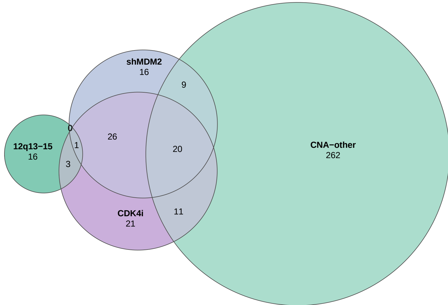
Figure 1B: 686 DE genes in WDLS vs normal fat (301 not in any set = 'Other genes with altered expression')
