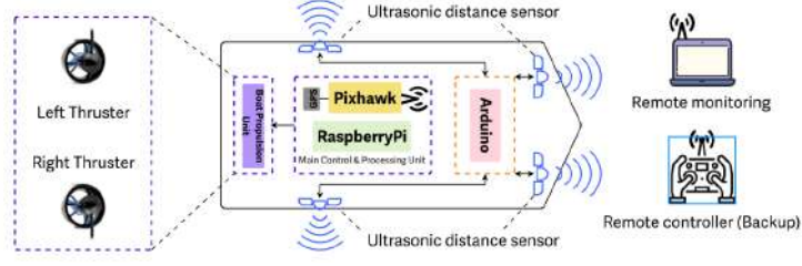
Fig. 3: System architecture
