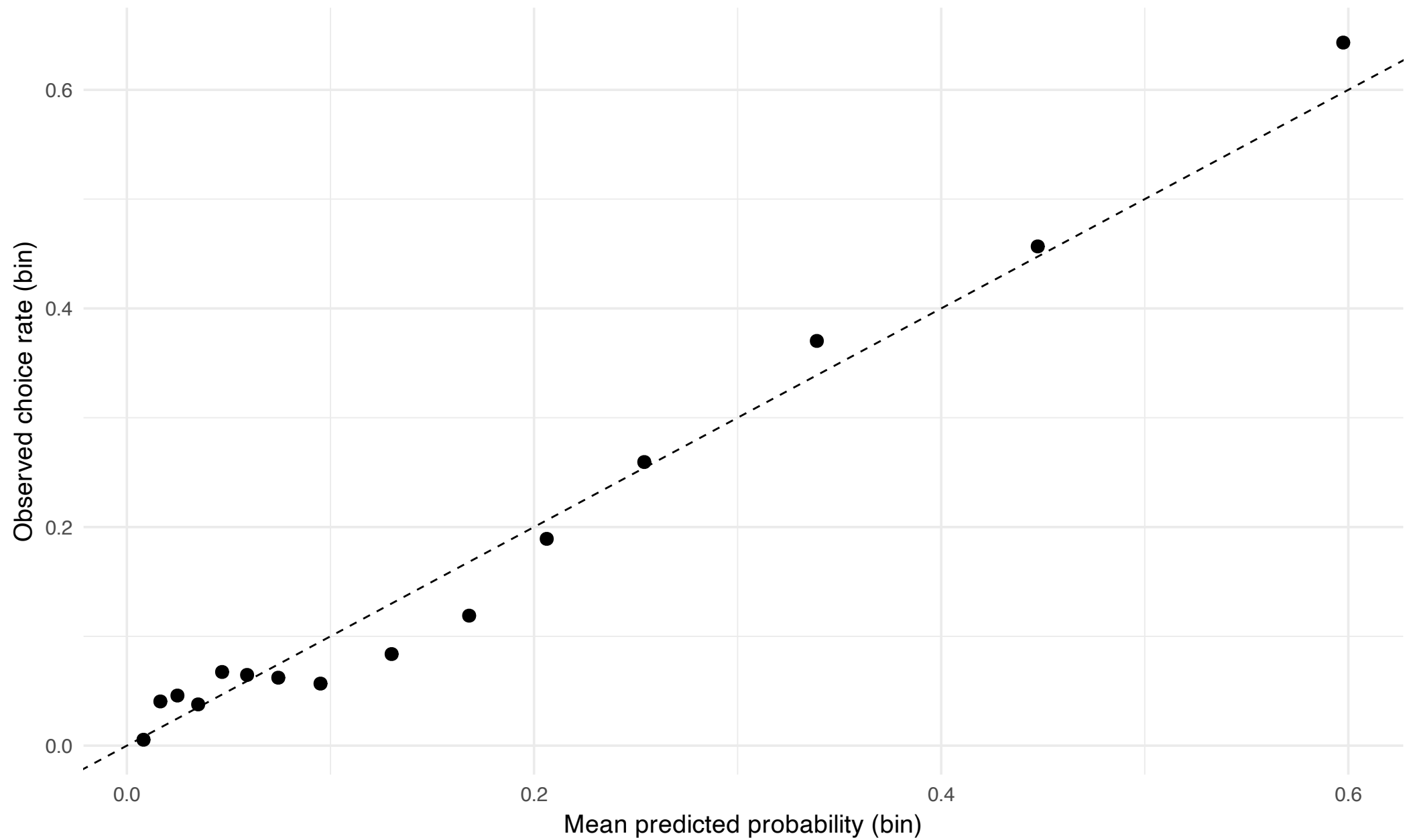
L3_learning: calibration (binned)
