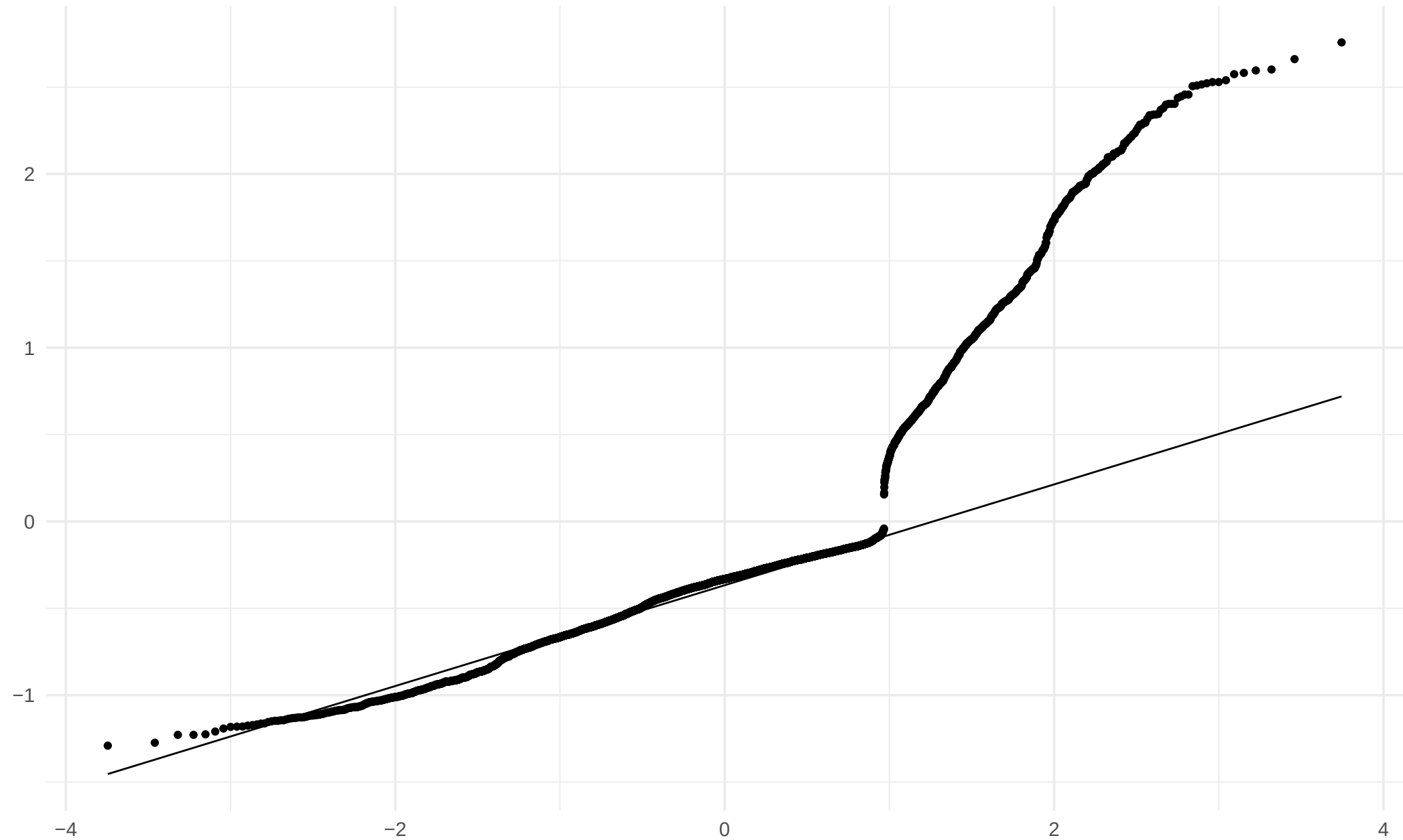
L3_learning: QQ deviance residuals
