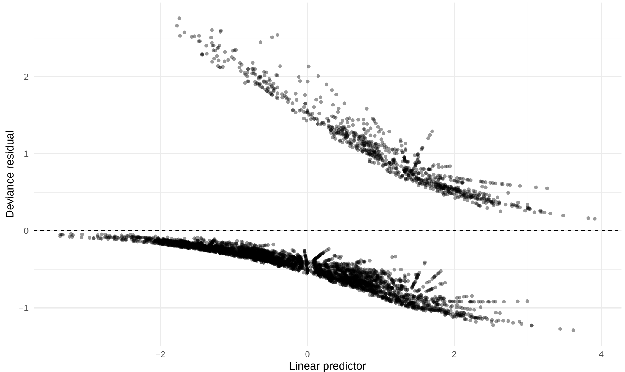
L3_learning: deviance residuals vs linear predictor
