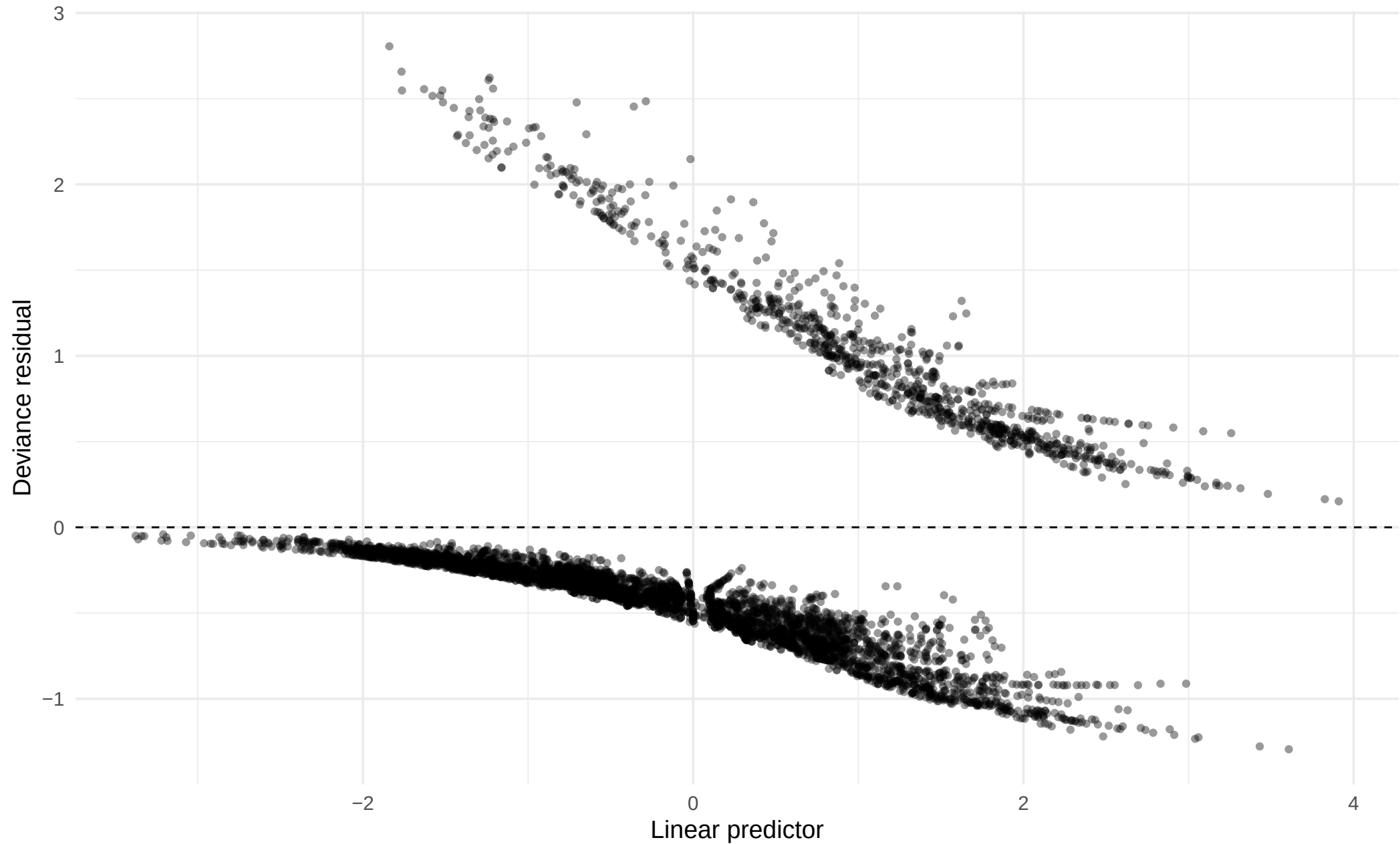
L5_Learning_clustered: deviance residuals vs linear predictor
