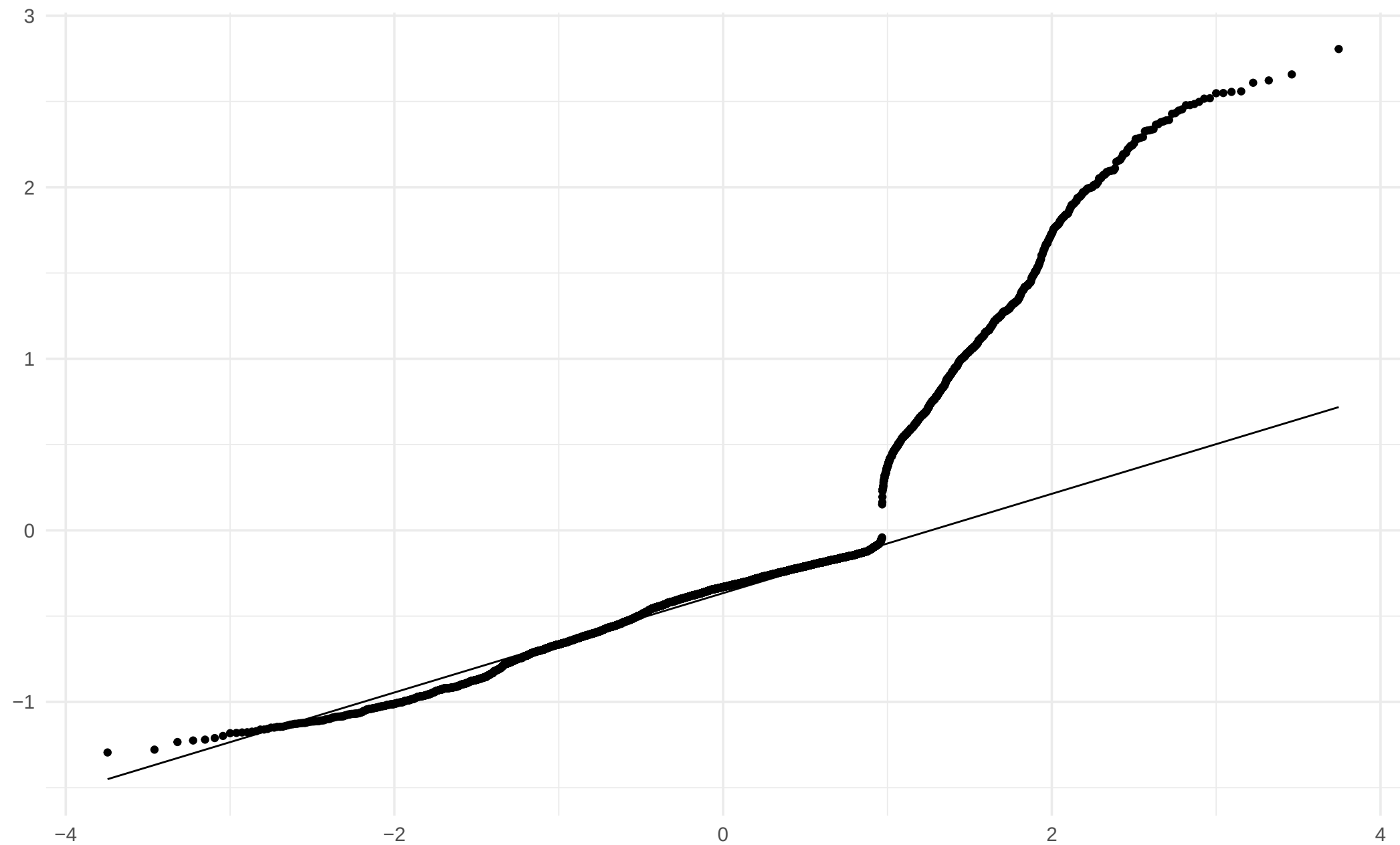
L5_Learning_clustered: QQ deviance residuals
