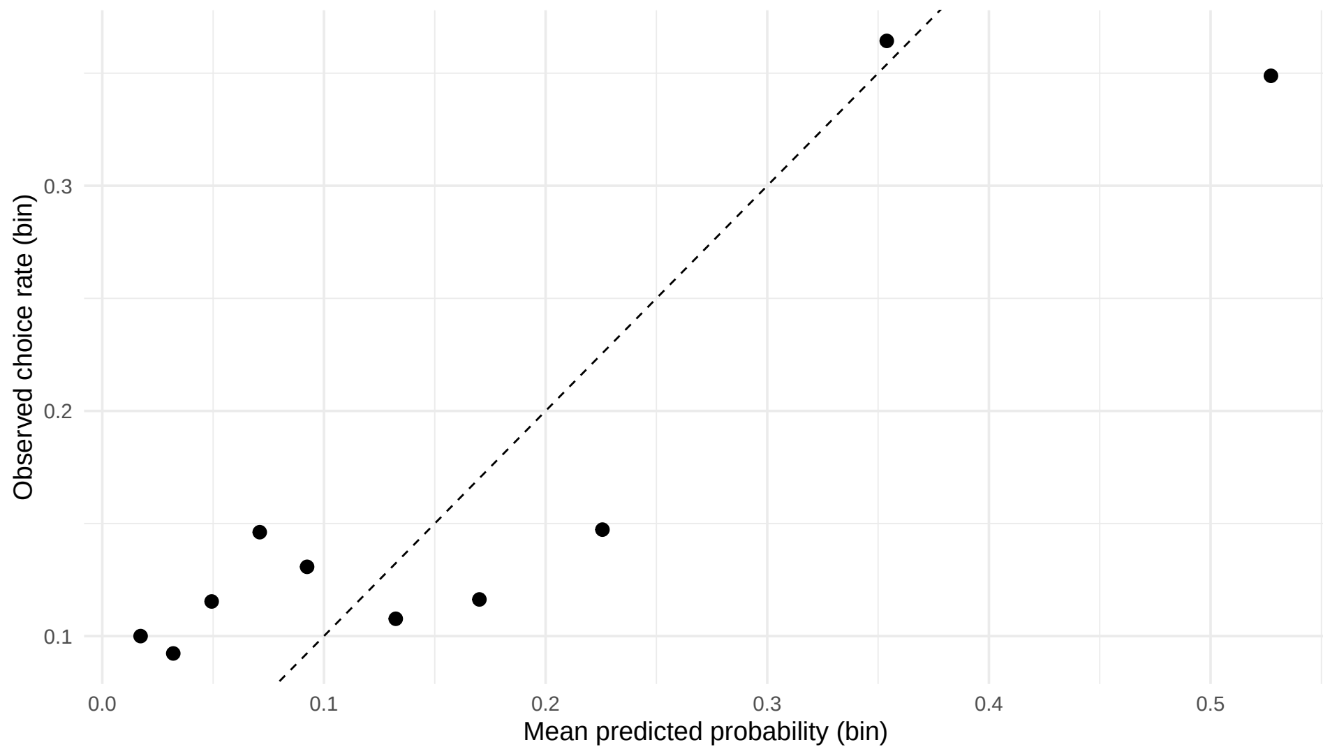
L5_learning_clustered: calibration (coinSet=A)
