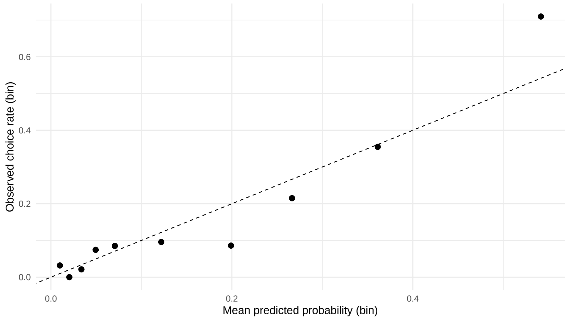
L5_learning_clustered: calibration (coinSet=B)
