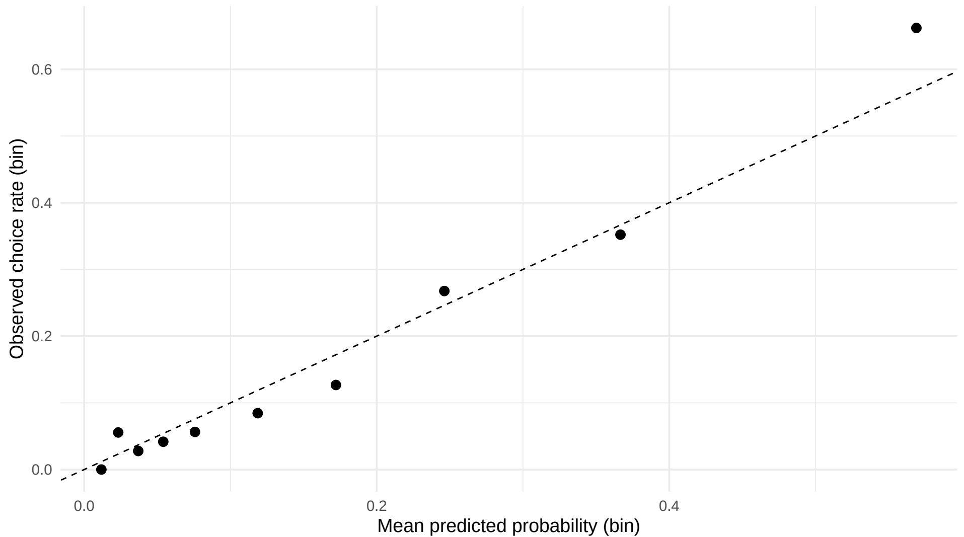
L5_learning_clustered: calibration (coinSet=Bx)
