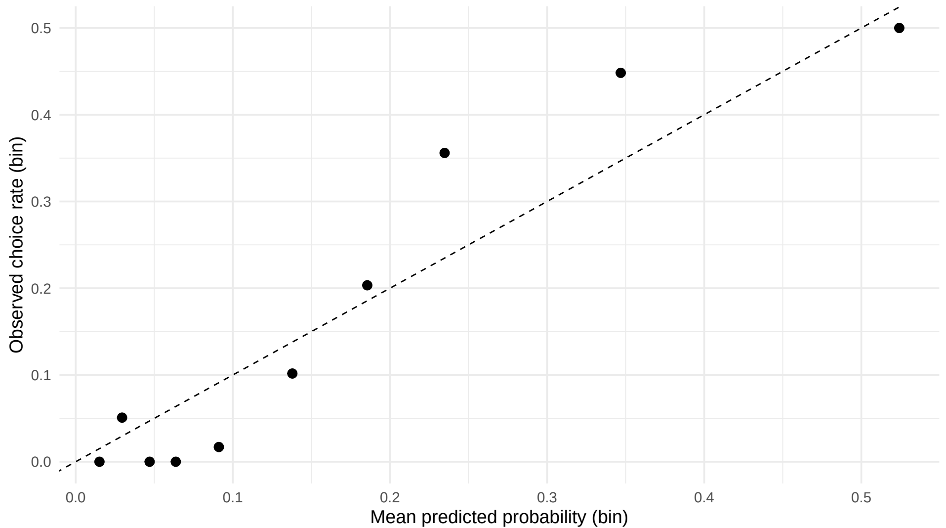
L5_learning_clustered: calibration (coinSet=D)
