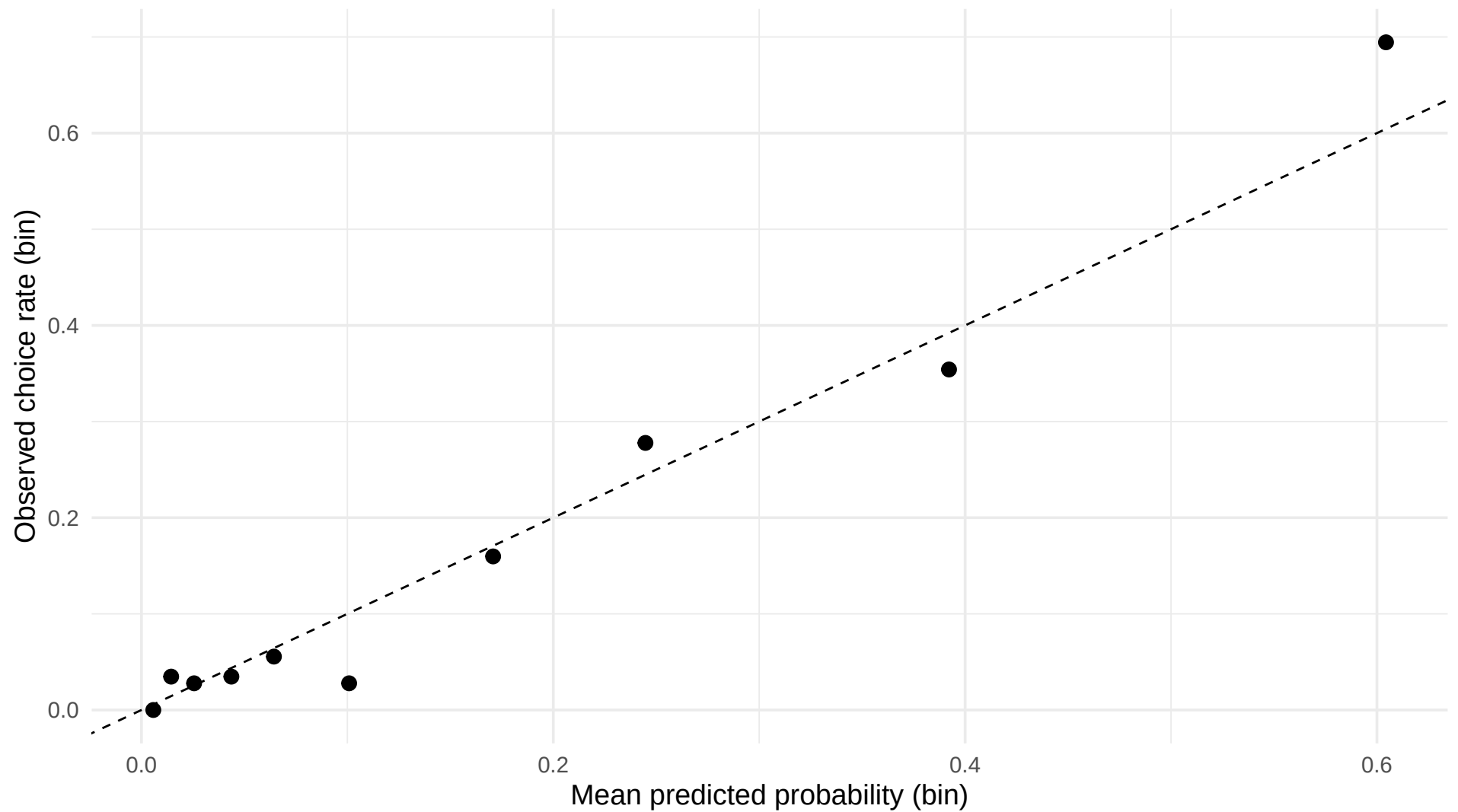
L5_learning_clustered: calibration (coinSet=Ax)
