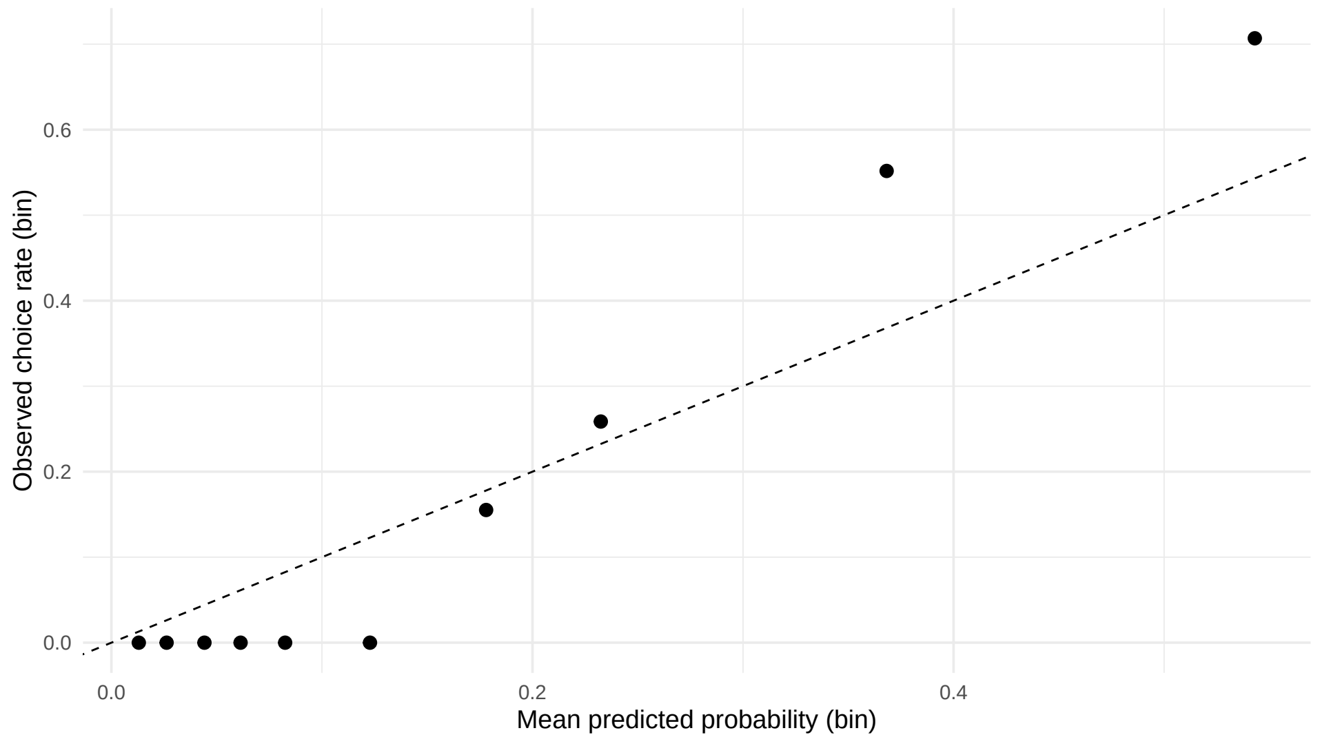
L5_learning_clustered: calibration (coinSet=C)
