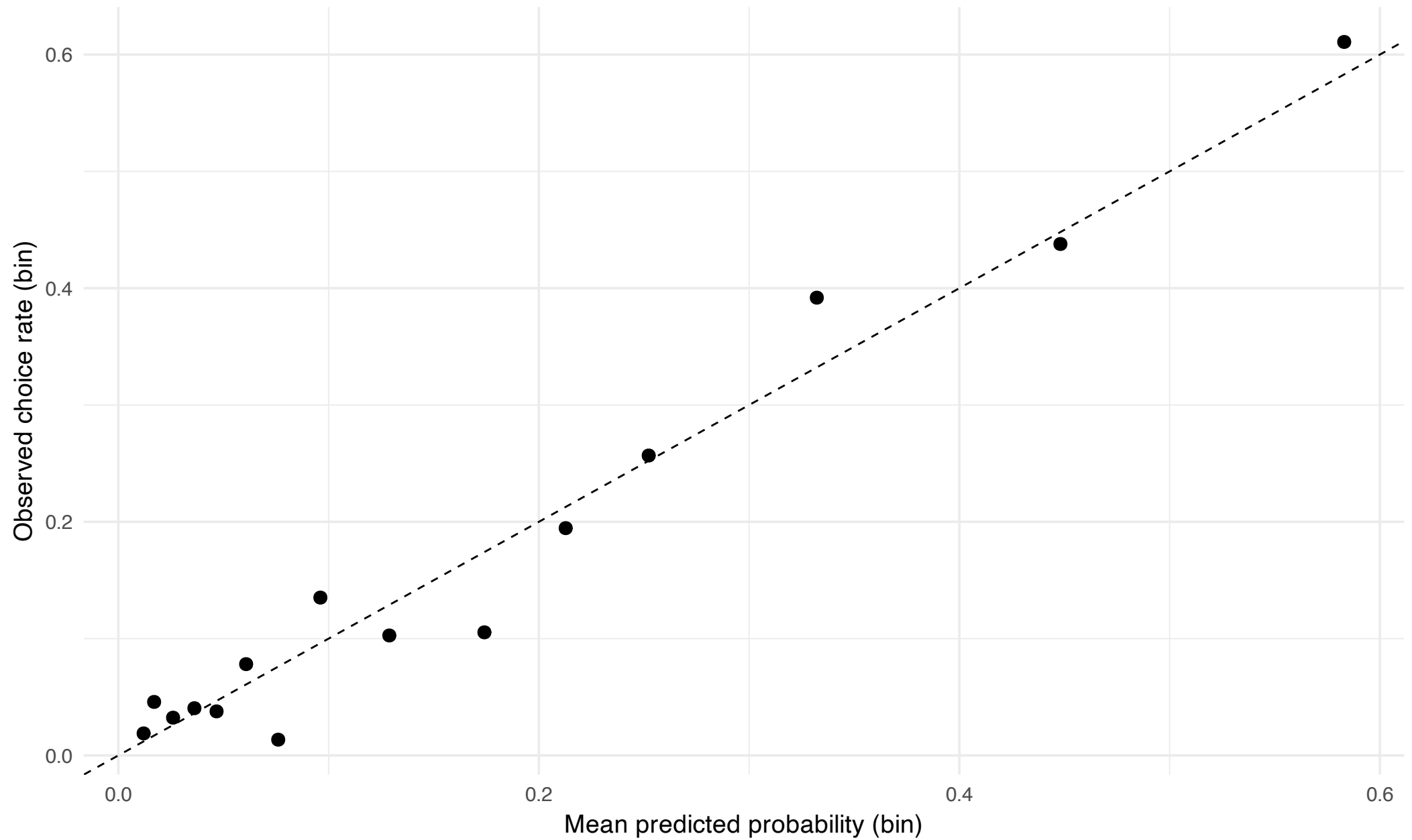
M3_value_distance: calibration (binned)
