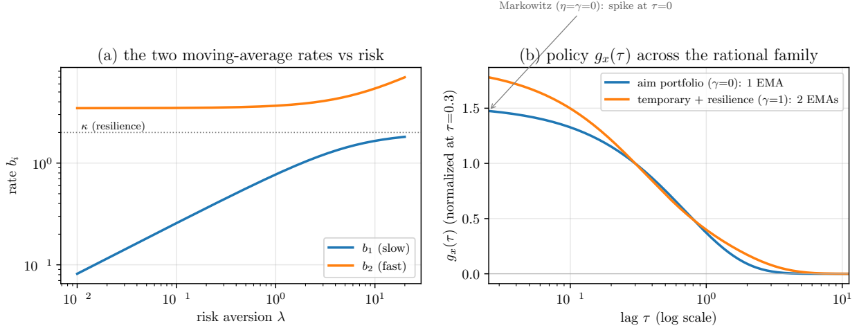
Figure 1: The rational friction family, at fixed \eta = 0.5 , \lambda = 1 , \theta = 1 . (a) For the temporary-plus-resilient friction ( \gamma = 1 , \kappa = 2 ), the two moving-average rates b_1, b_2 against risk aversion \lambda : the slow rate b_1 tends to zero as \lambda \rightarrow 0 , where the position becomes non-stationary, while the fast rate stays near the resilience \kappa . (b) The lag-domain position impulse response g_x(\tau) (normalized at \tau = 0.3 ) across the family: the aim portfolio ( \gamma = 0 ) is a single exponential moving average, the temporary-plus-resilient friction ( \gamma = 1 ) a sum of two, and the memoryless Markowitz limit ( \eta = \gamma = 0 ) a spike at zero lag. All are finite-memory; the power-law kernel and its algebraic tail appear in Figure 2.
