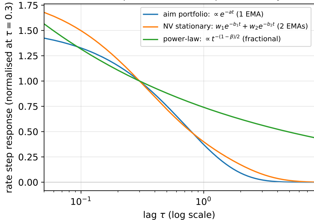
(b) rate in response to unit step in \alpha (analytical)
