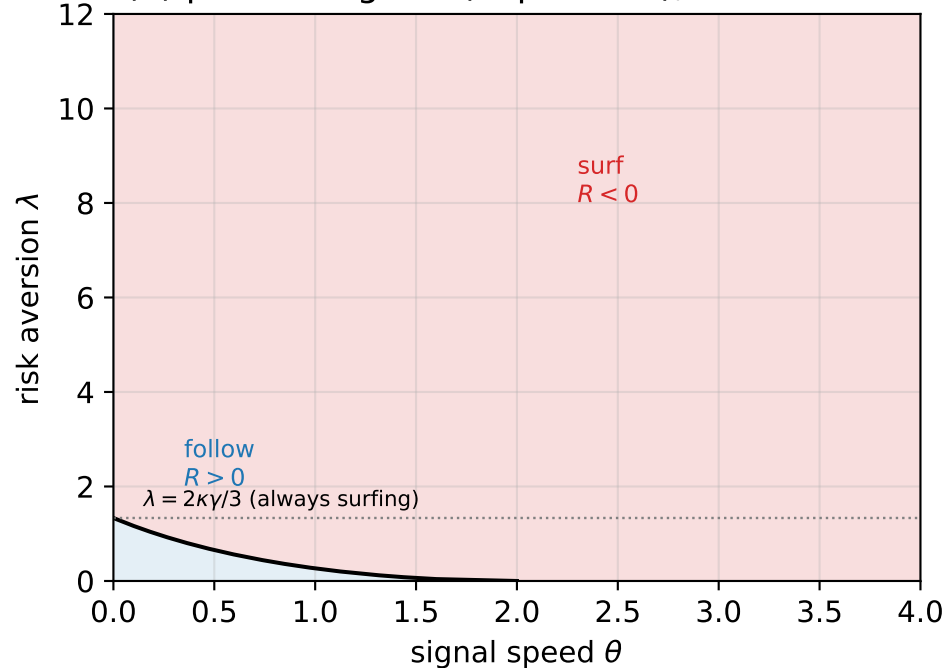
(b) phase diagram (exp kernel), \theta^* = \kappa - 2m
