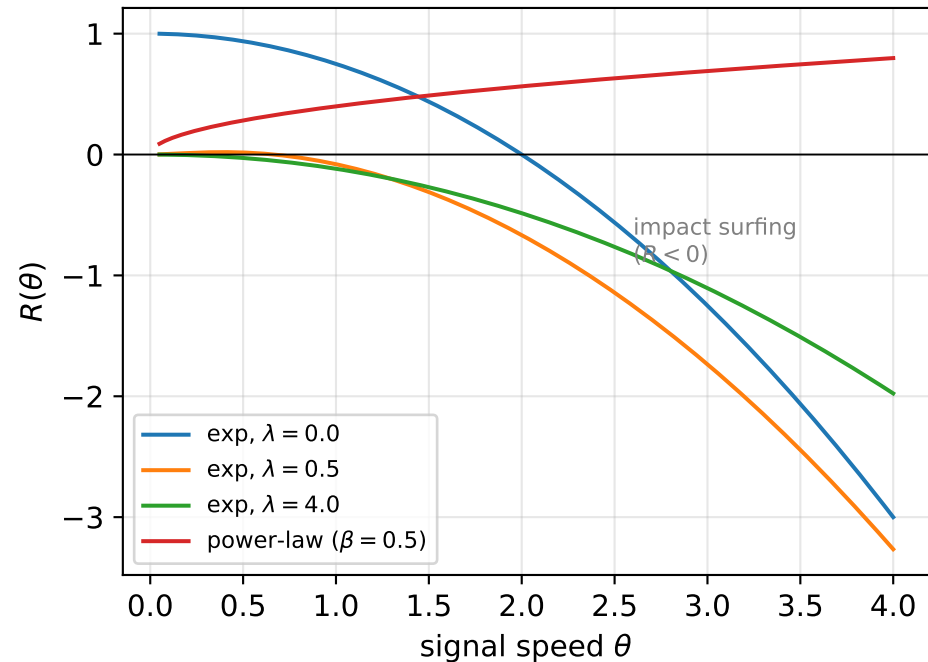
(a) flow response R(\theta)
