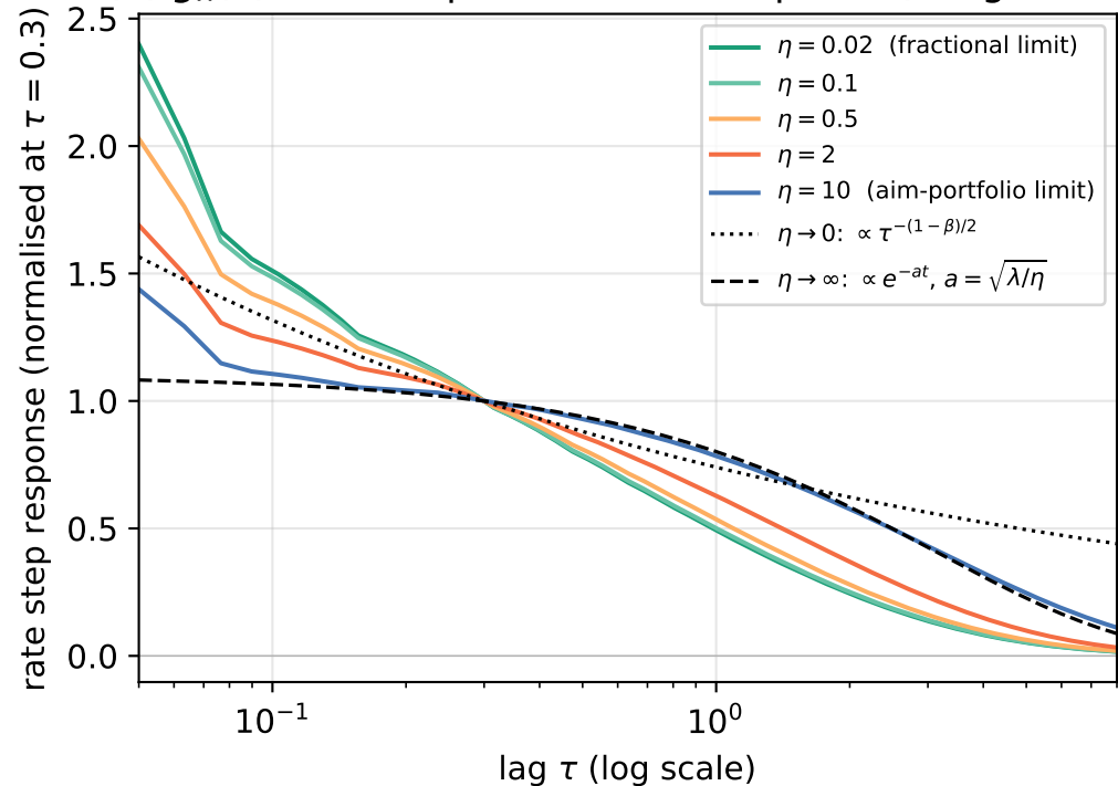
(b) g_x(\tau) : rate response to unit step in \alpha (Szegő filter)
