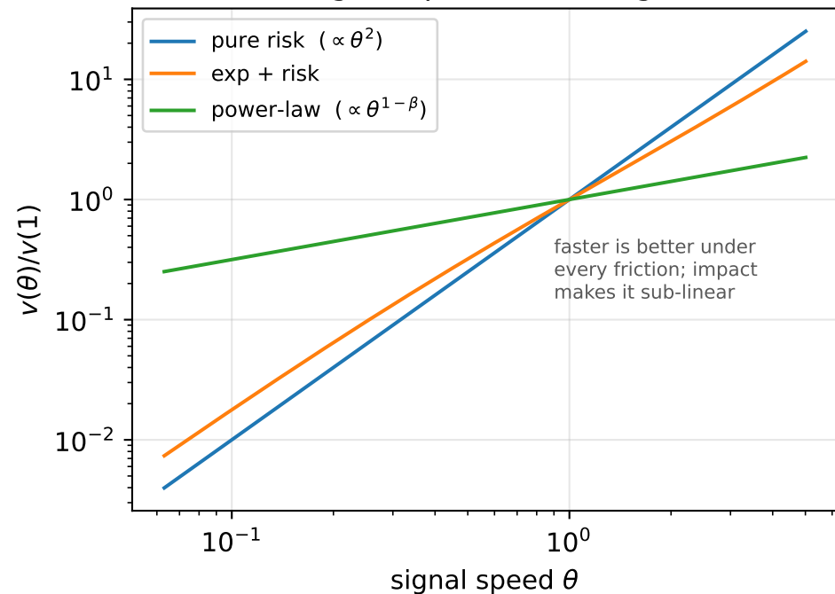
(a) value vs signal speed (fixed signal variance)
