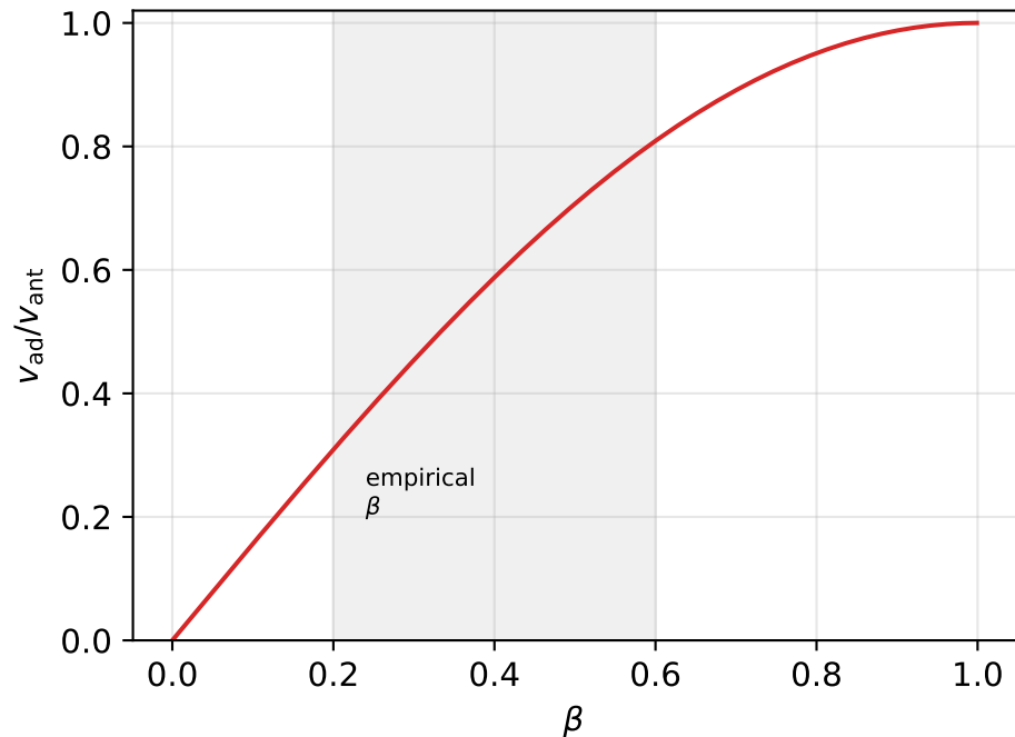
(b) cost of causality: v_{\text{ad}}/v_{\text{ant}} = \sin(\pi\beta/2)
