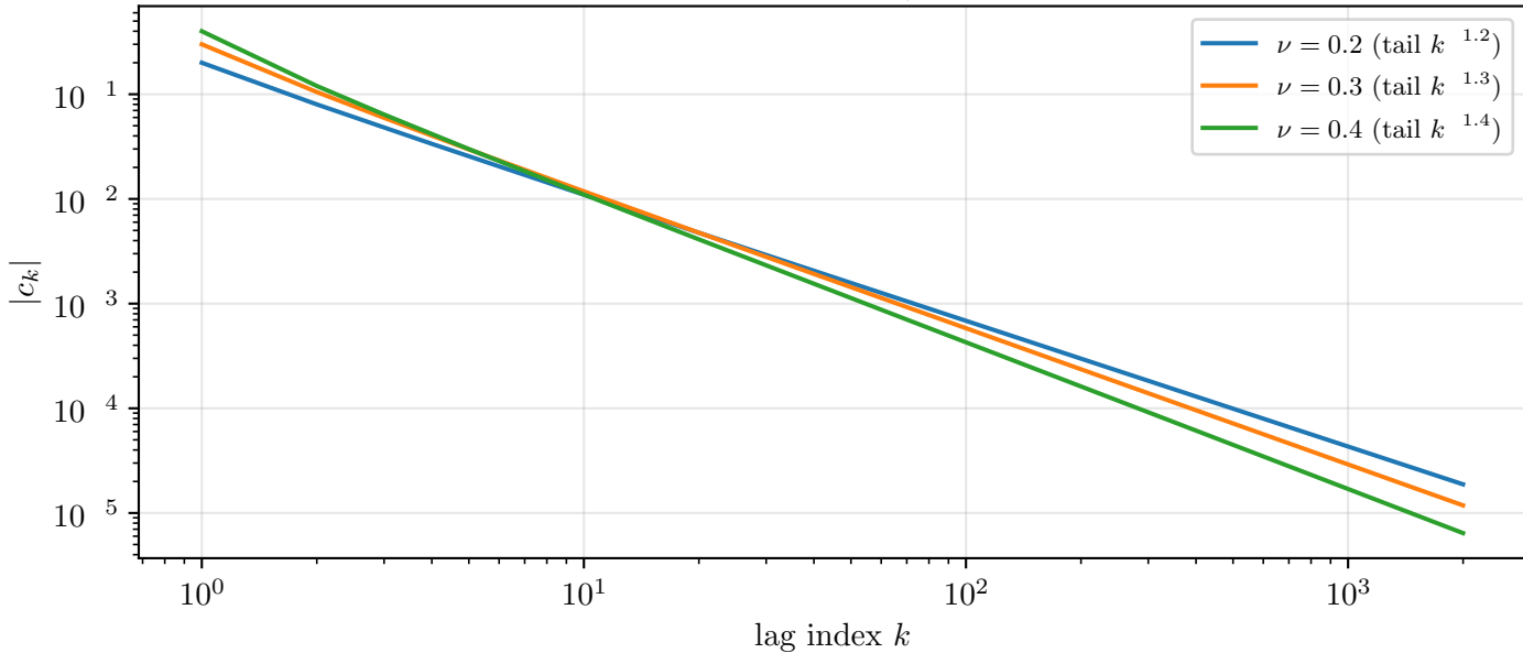
Fractional-derivative weights D_+^\nu (Grünwald–Letnikov)
