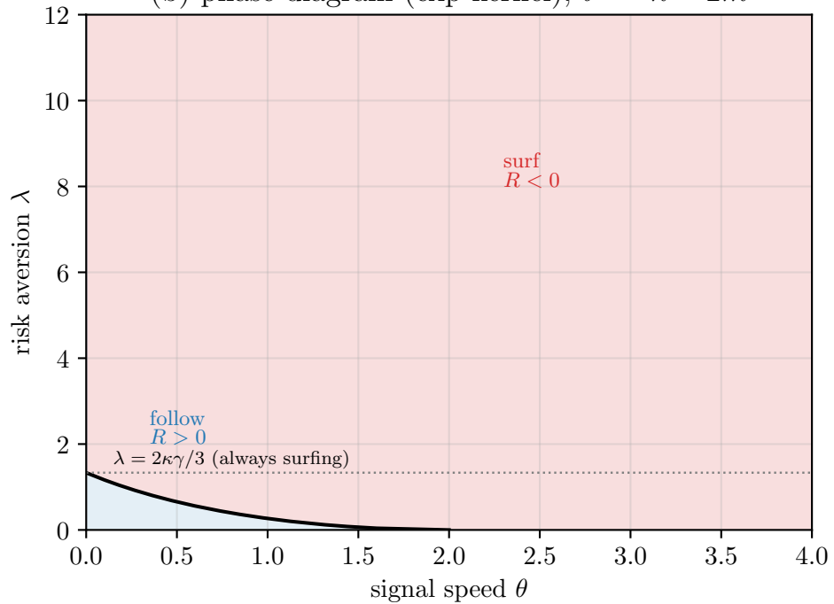
(b) phase diagram (exp kernel), \theta^* = \kappa / 2m
