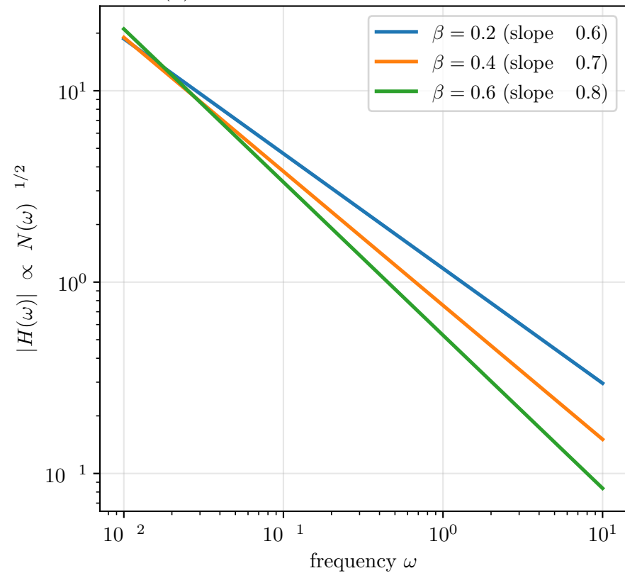
(a) power-law impact: fractional filter
