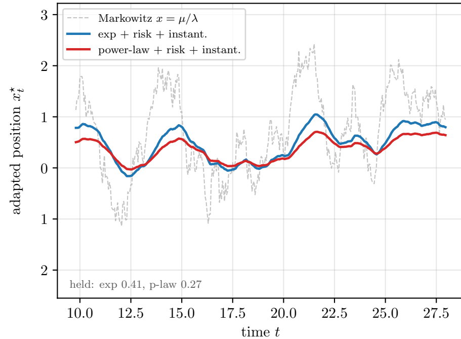
\theta = 0.5 (slow, \theta < \kappa )
