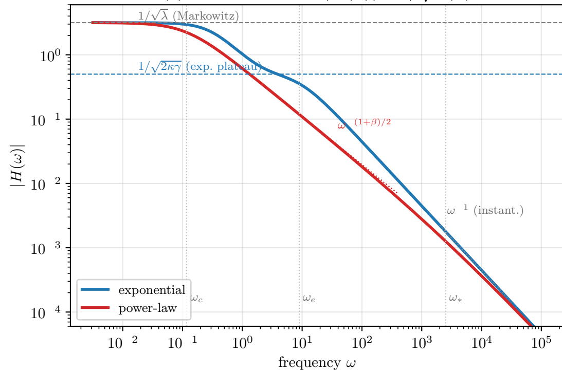
(a) transfer function |H(\omega)| = 1/\sqrt{n(\omega)}
