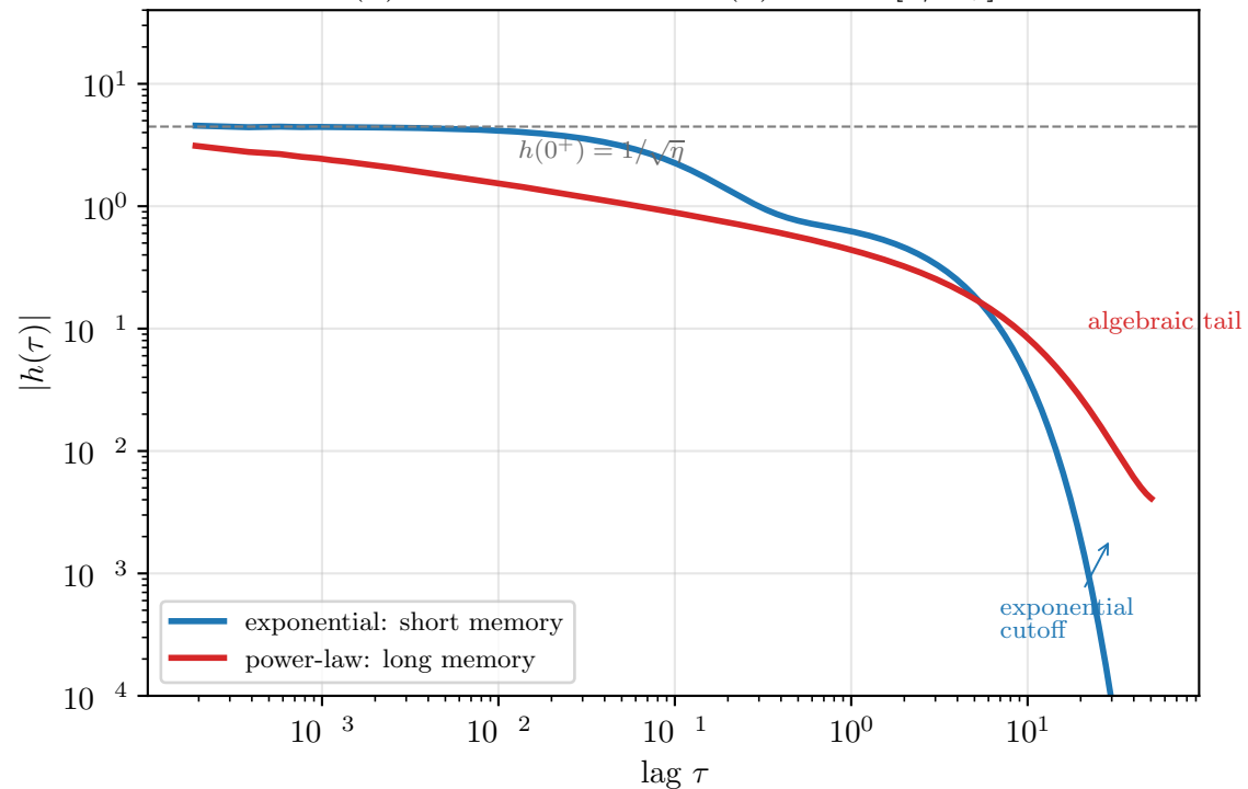
(b) impulse response h(\tau) = \mathcal{F}^{-1}[1/n_+]
