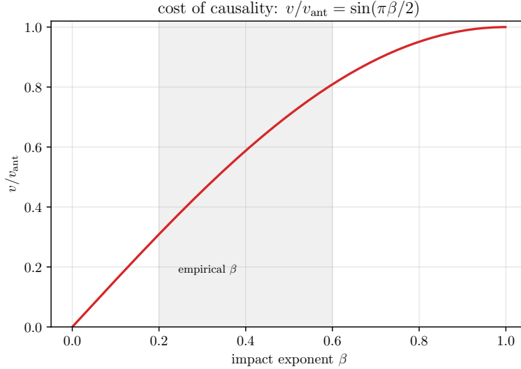
Figure 5: The causality gap under power-law impact. The adapted value is a fixed fraction v/v_{\text{ant}} = \sin(\pi\beta/2) of the perfect-foresight value, independent of the signal speed; the shaded band marks the empirical range of \beta .
