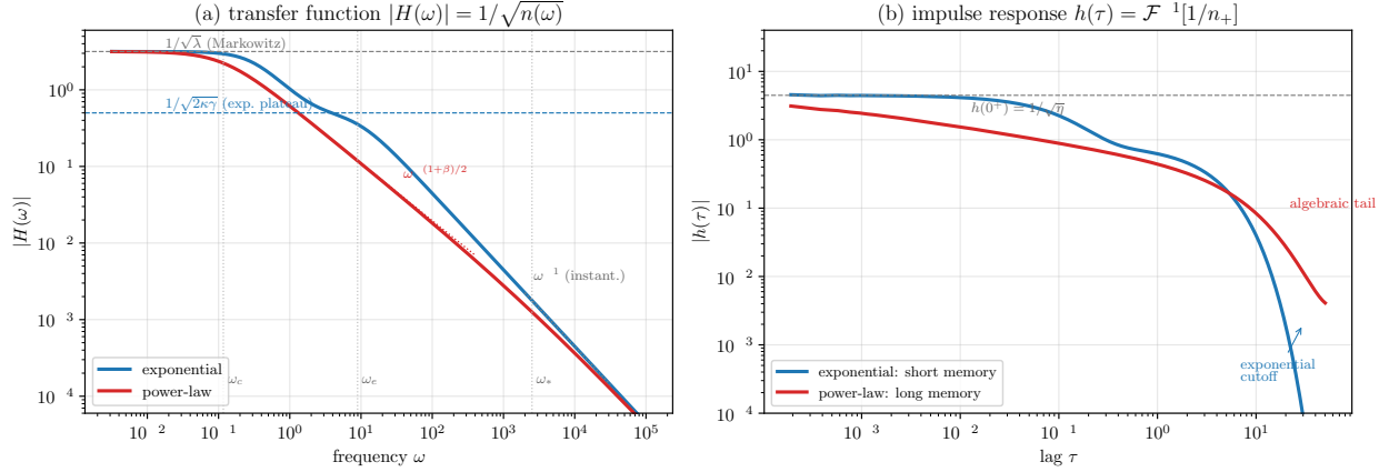
Figure 4: The trading filter for exponential versus power-law transient impact ( \gamma = 1 , \kappa = 2 , \beta = 0.5 ; small \lambda = 0.1 , \eta = 0.05 ). (a) Transfer function |H(\omega)| = 1/\sqrt{\hat{n}(\omega)} : both share the low-frequency Markowitz plateau and roll off as \omega^{-1} under the instantaneous cost at high frequency; between them the exponential settles on a finite-memory plateau while the power law slides as \omega^{-(1+\beta)/2} . (b) Impulse response h(\tau) = \mathcal{F}^{-1}[\hat{n}_+^{-1}] : the exponential filter cuts off past the instantaneous-cost scale, the power law leaves an algebraic tail.
