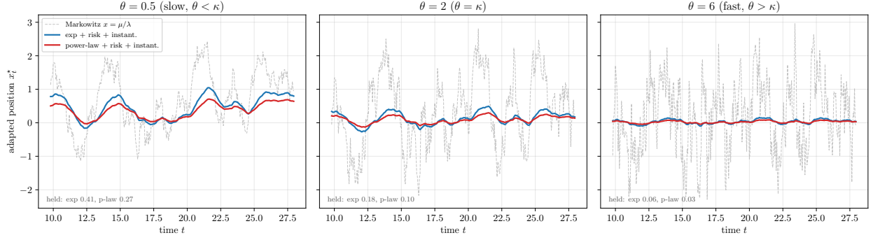
Figure 2: Adapted position across signal speeds, on a common Ornstein–Uhlenbeck path ( \gamma = 1 , \kappa = 2 , \beta = 0.5 , \lambda = 1 , \eta = 0.5 ; interior window, unit return variance). As the mean-reversion rate \theta rises from below to above the resilience \kappa , the optimal position tracks a smaller and smoother fraction of the frictionless Markowitz position \mu/\lambda (dashed); the retained fraction of its magnitude is annotated in each panel. Less is held under power-law impact than under exponential impact of equal strength.
