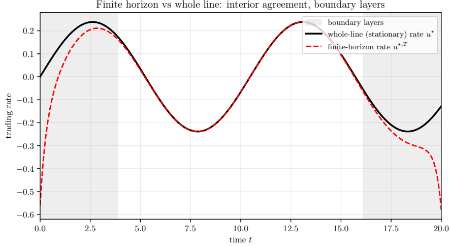
Figure 6: Finite horizon versus whole line ( \eta = 0.5 , \gamma = 1 , \kappa = 2 , \lambda = 1 , T = 20 ), on a deterministic sinusoidal signal so that only the boundary layers distinguish the two. The finite-horizon optimal rate follows the whole-line stationary rate through the interior and departs only in the start-up and terminal boundary layers of Proposition 1; the shading marks three e-folds of the slowest rate b_1 , a scale rather than a fitted width.
