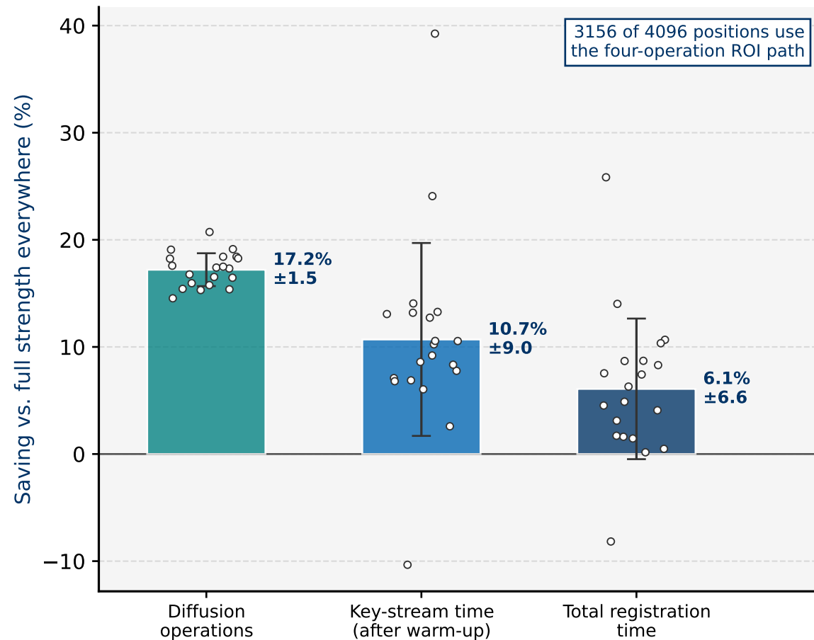
Measured Saving (n = 20 BraTS slices; mean \pm SD)
