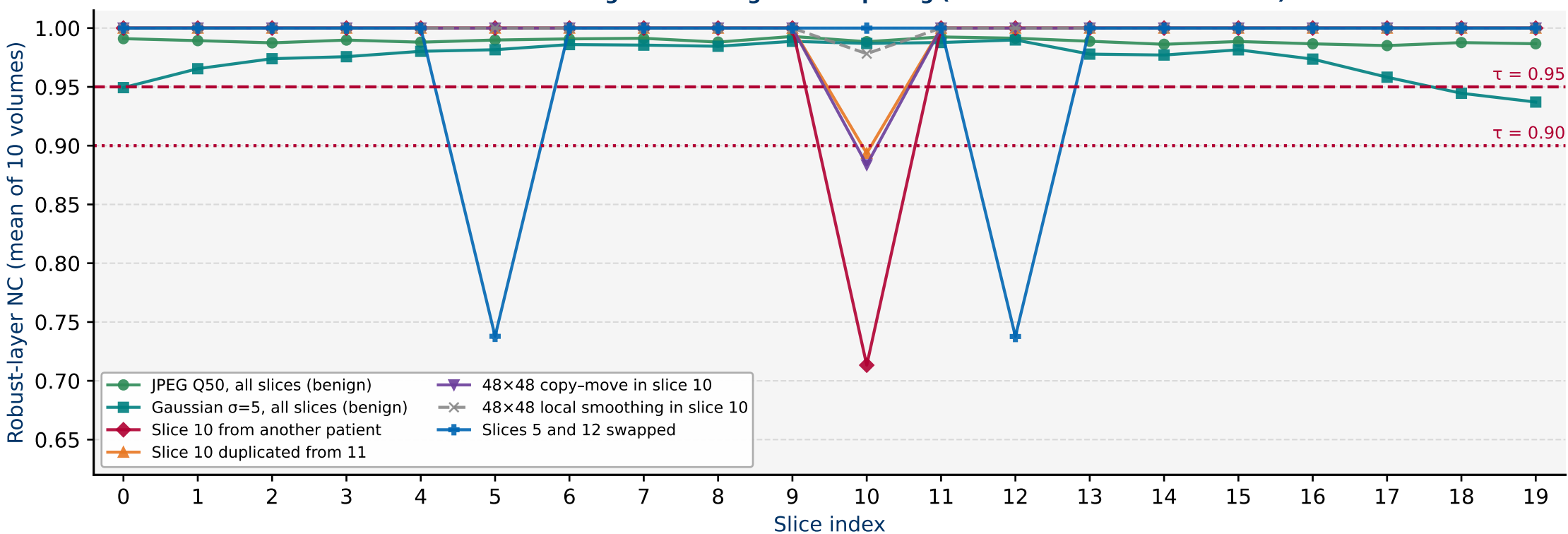
Per-Slice NC for Benign Processing and Tampering (10 BraTS volumes × 20 slices)
