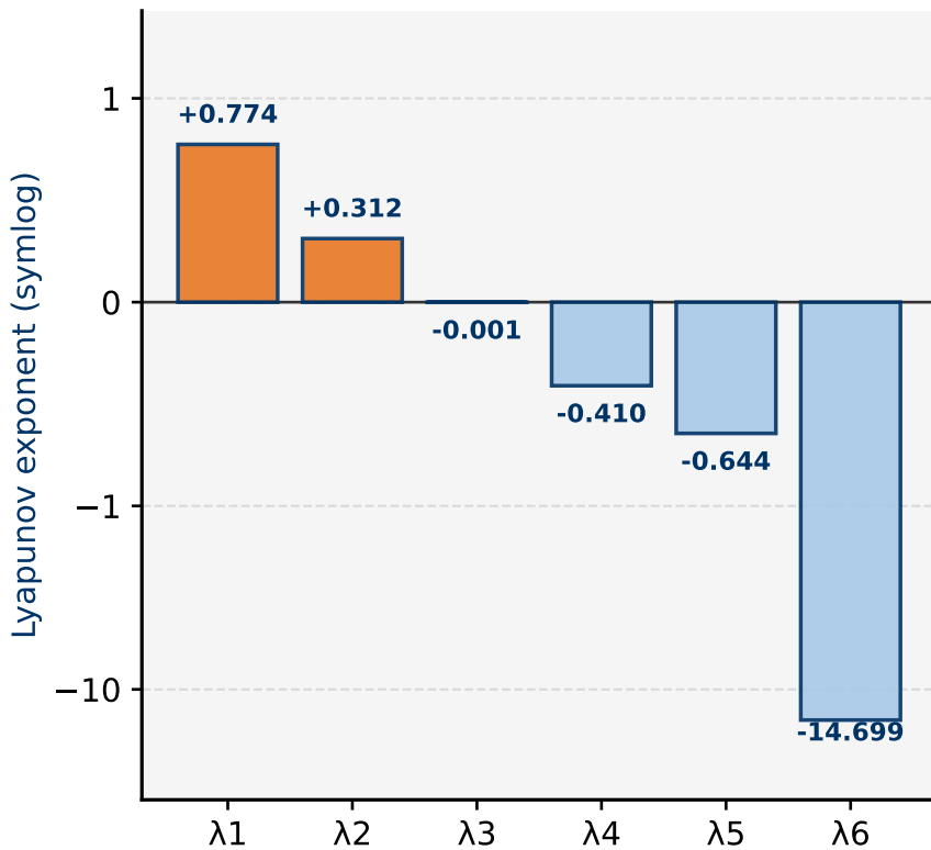
(a) Lyapunov Spectrum of the 6D System two positive exponents \rightarrow hyperchaotic
