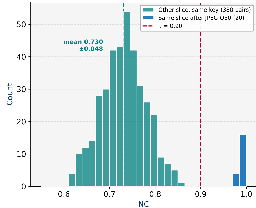
(c) Distinguishability on BraTS
