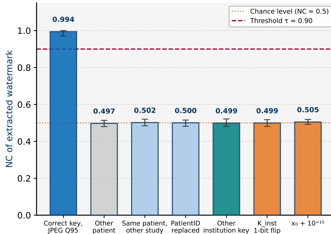
(b) Key Sensitivity on TCIA (26 slices; whiskers: min-max)
