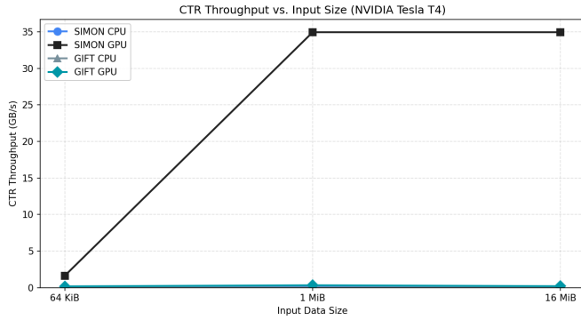
Fig. 1. CTR throughput (GB/s) vs. input size on NVIDIA Tesla T4 (SM 7.5, nvcc -O2).
