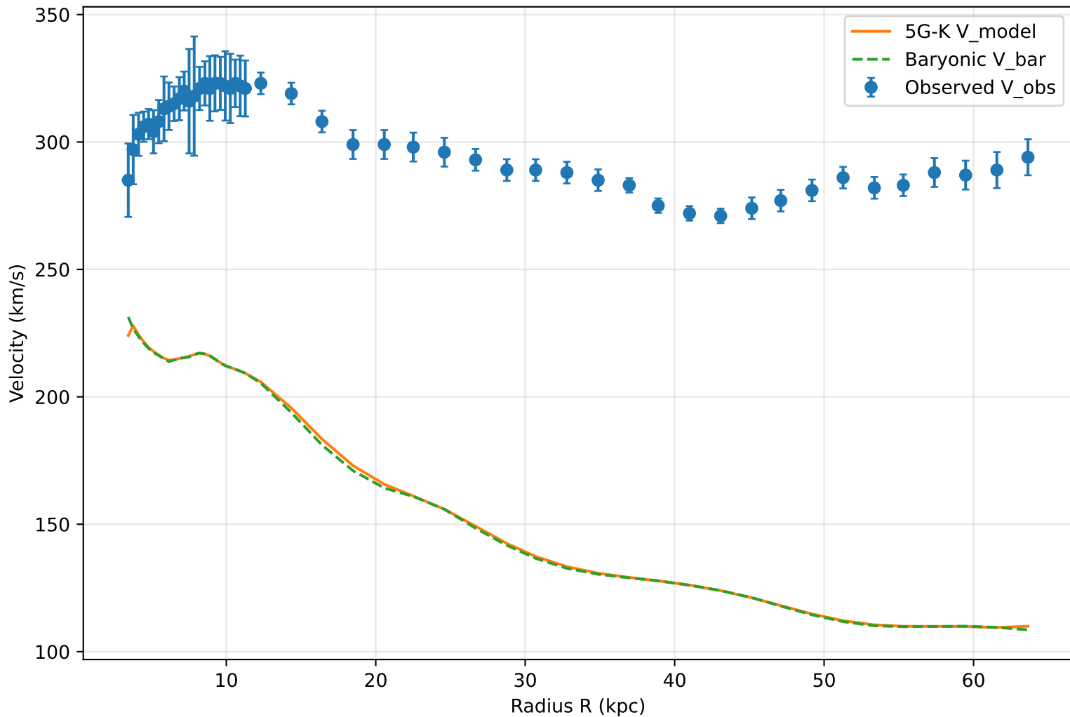
5G-K Variational Scheduler: NGC2841
