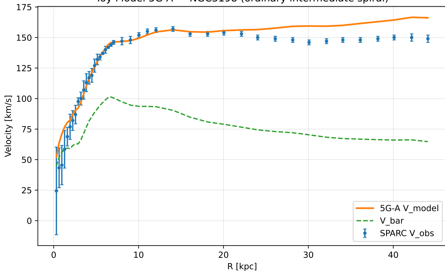
Toy Model 5G-A — NGC3198 (ordinary intermediate spiral)
