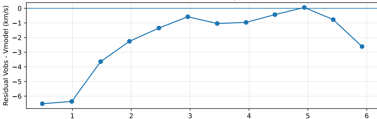
5G-F Residual and Nonlocal Response: DDO154
