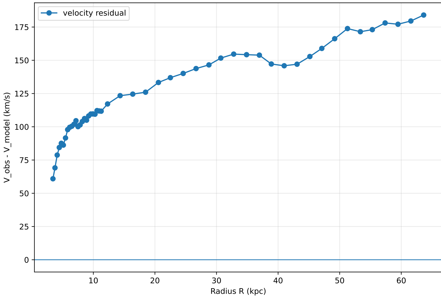
5G-K residual: NGC2841
