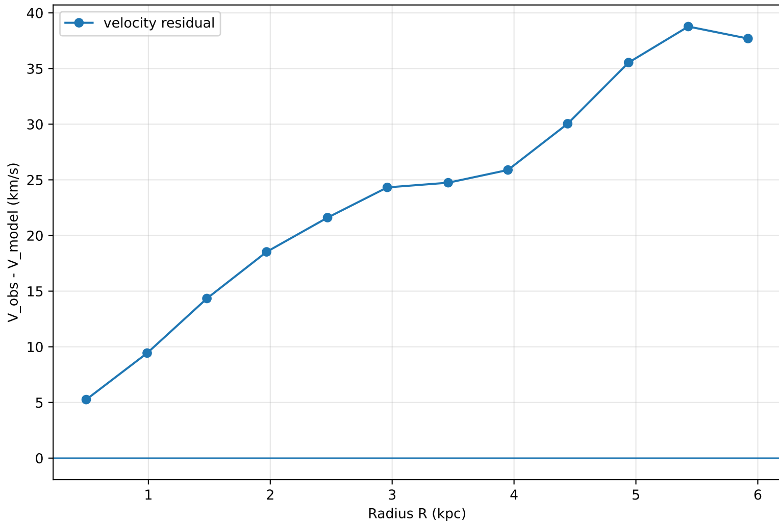
5G-K residual: DDO154
