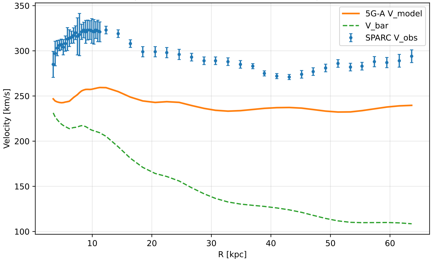
Toy Model 5G-A — NGC2841 (massive spiral)
