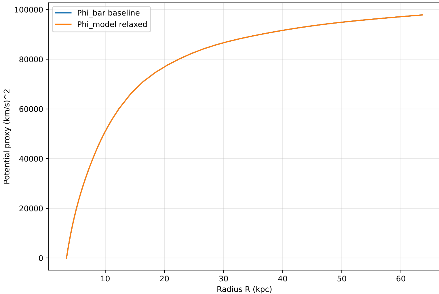
Potential field relaxation: NGC2841
