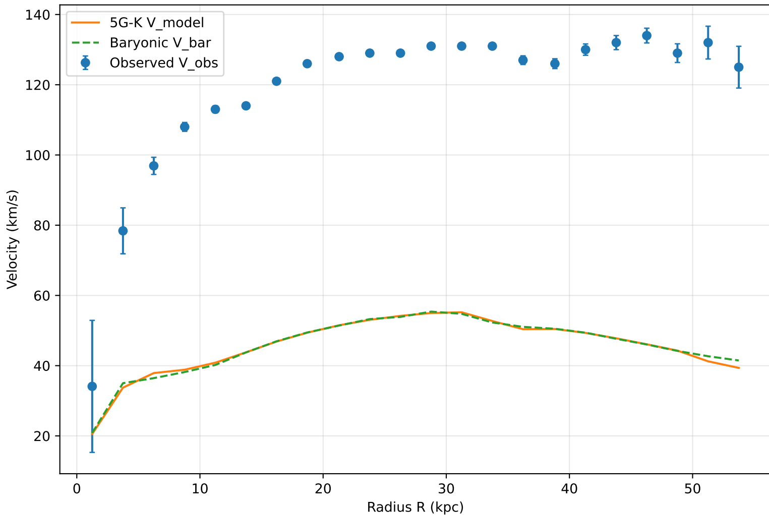
5G-K Variational Scheduler: UGC00128
