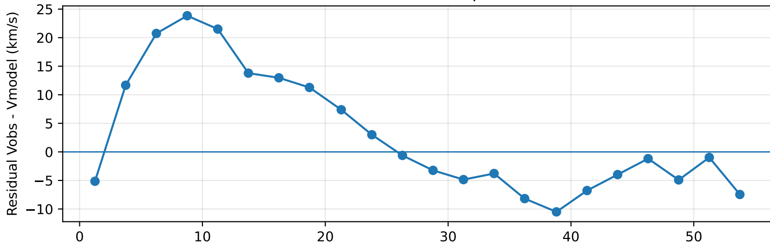
5G-F Residual and Nonlocal Response: UGC00128
