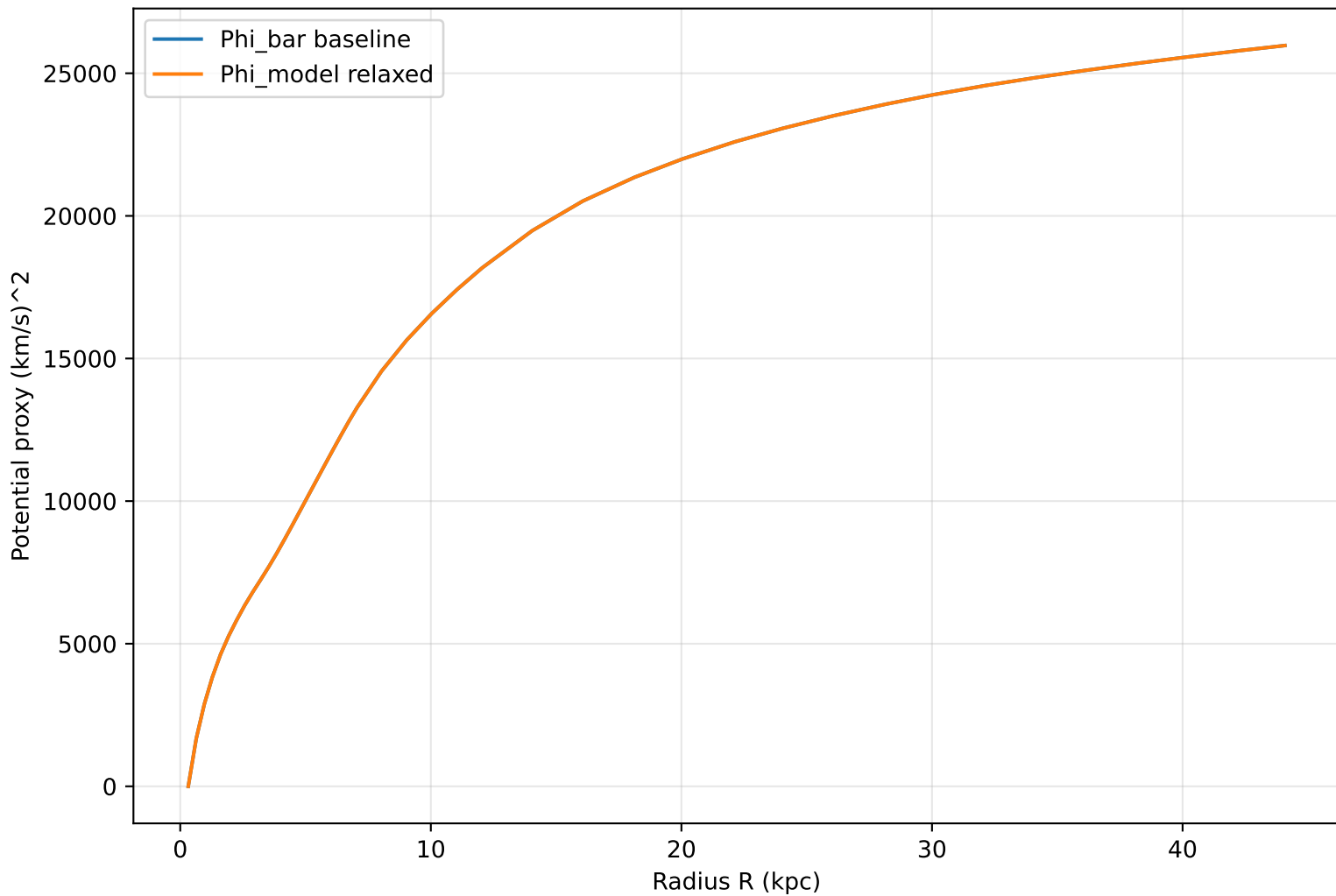
Potential field relaxation: NGC3198
