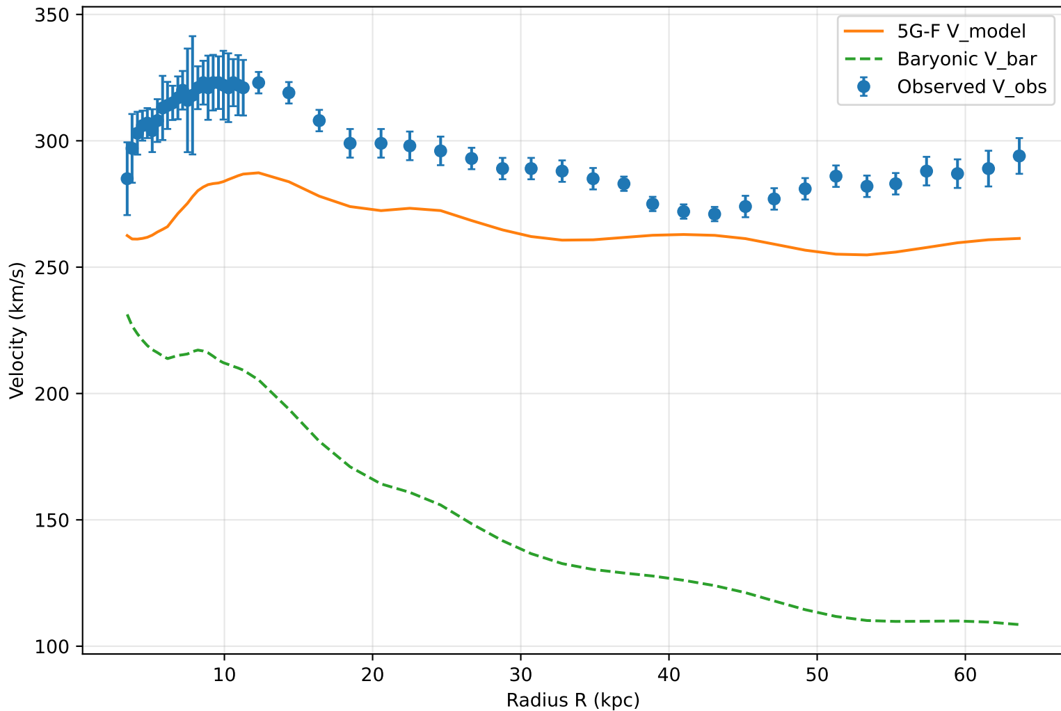
5G-F Nonlocal Kernel: NGC2841
