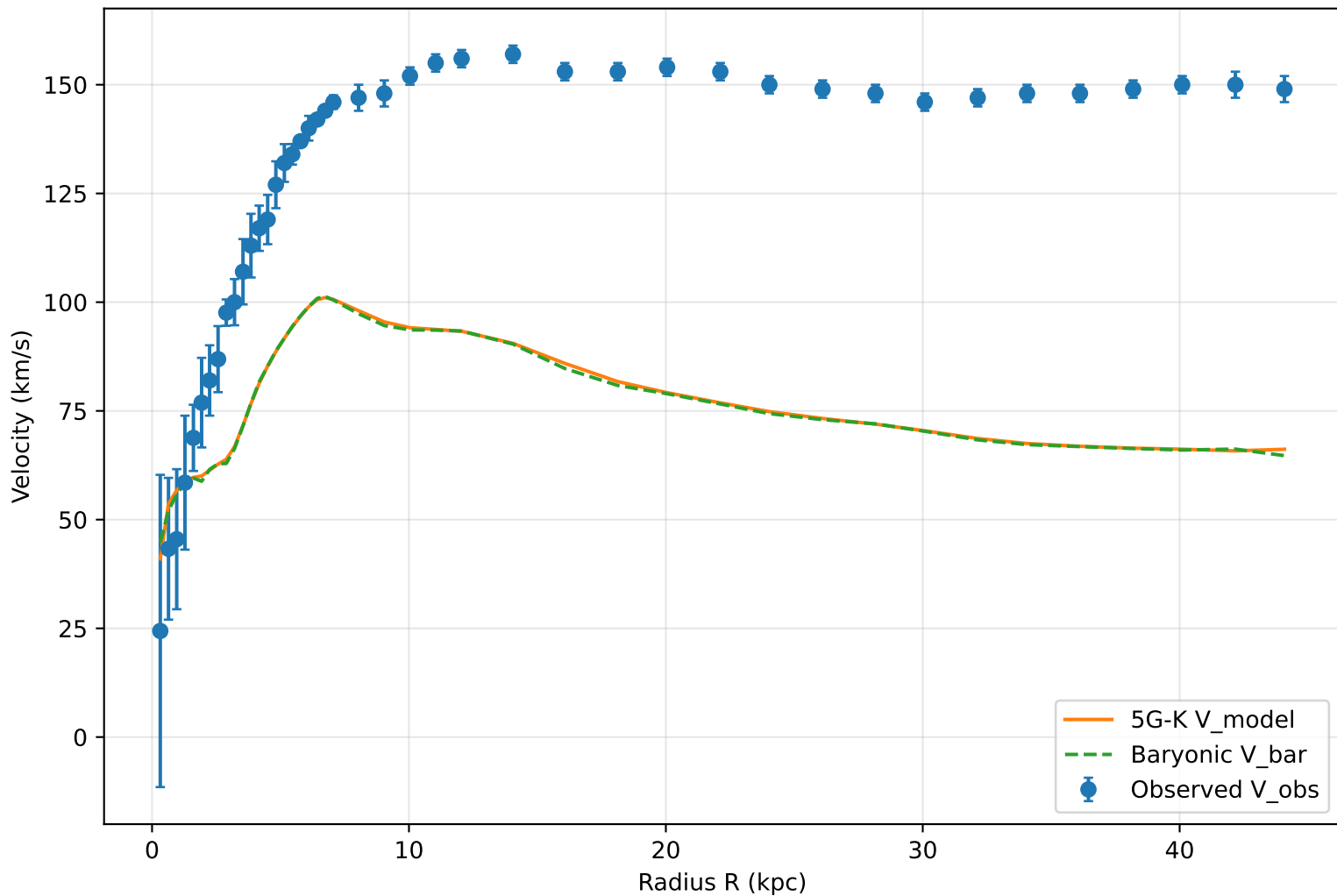
5G-K Variational Scheduler: NGC3198
