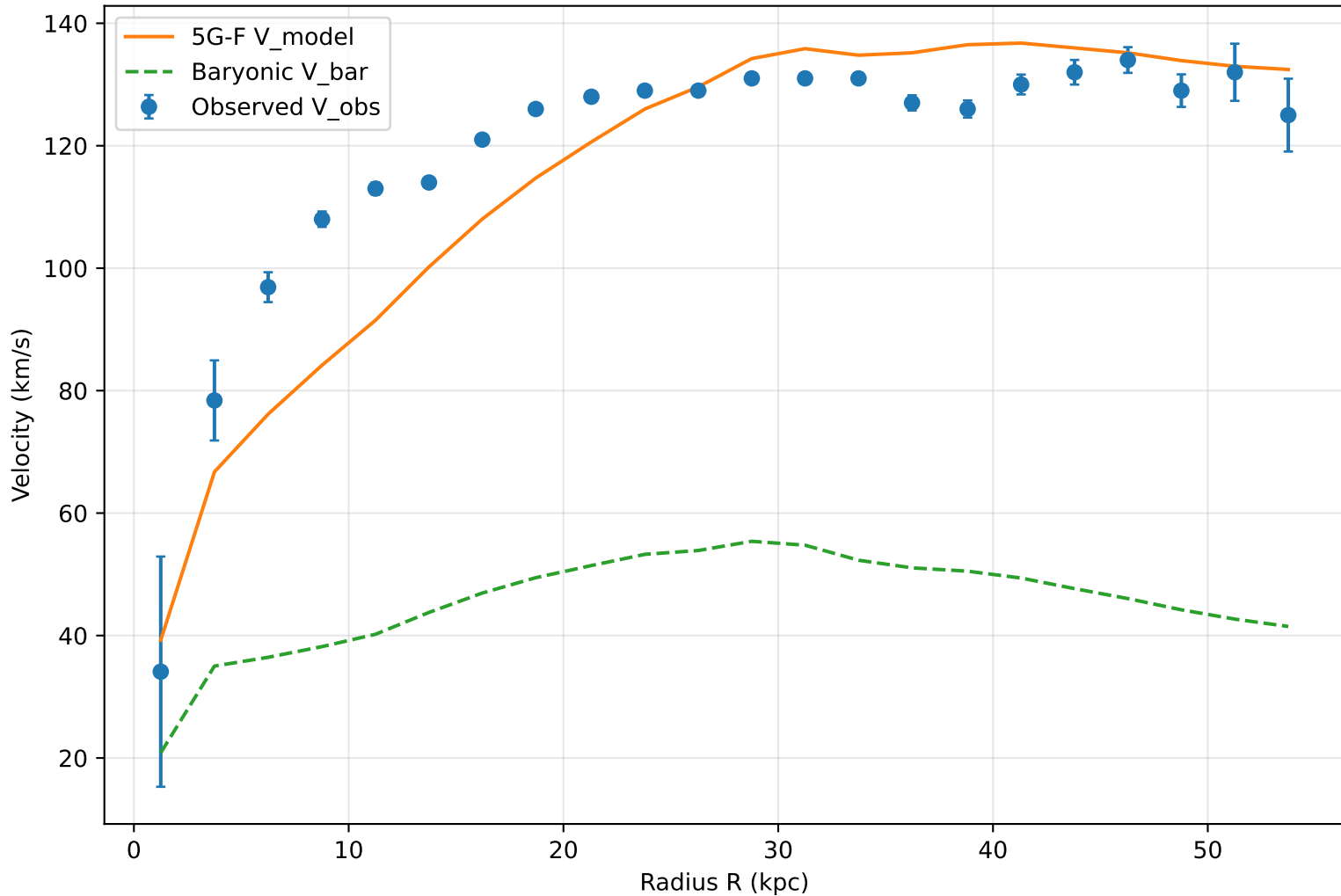
5G-F Nonlocal Kernel: UGC00128
