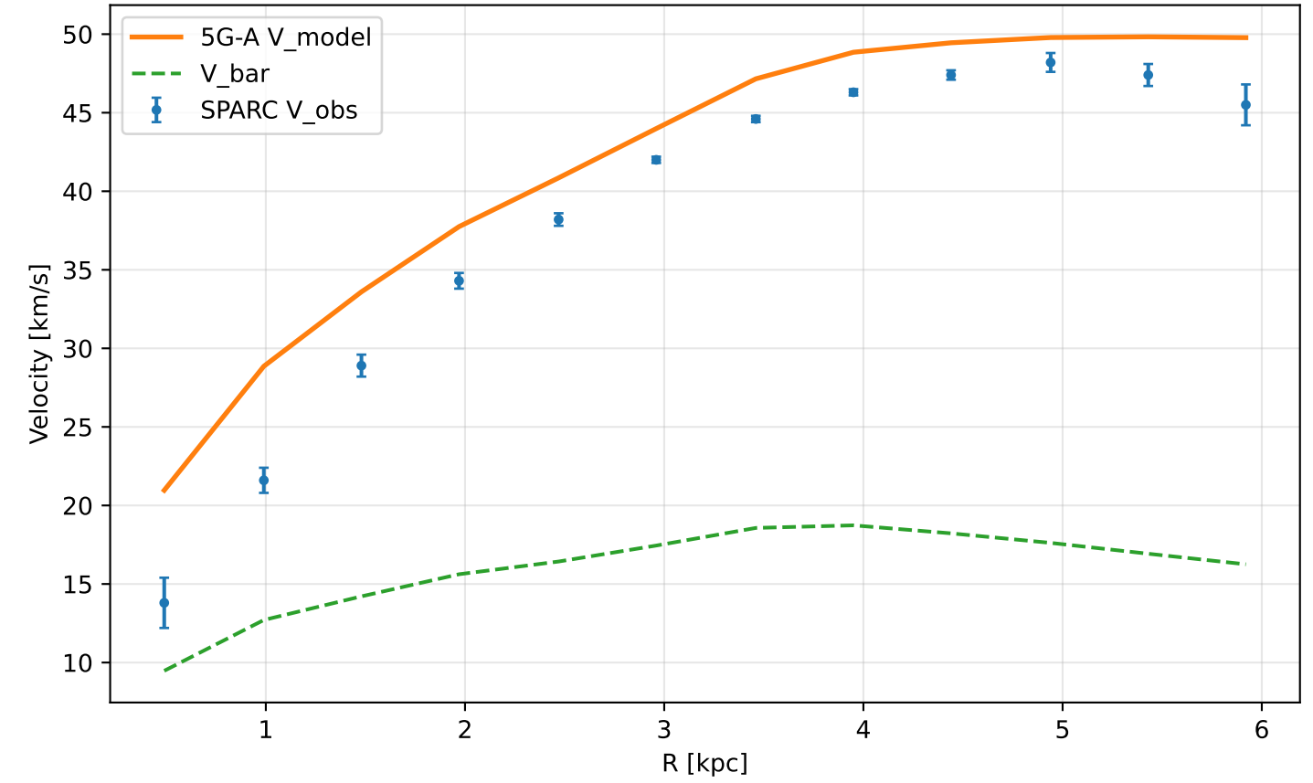
Toy Model 5G-A — DDO154 (gas-rich dwarf)
