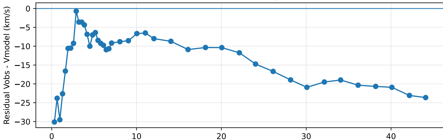
5G-F Residual and Nonlocal Response: NGC3198
