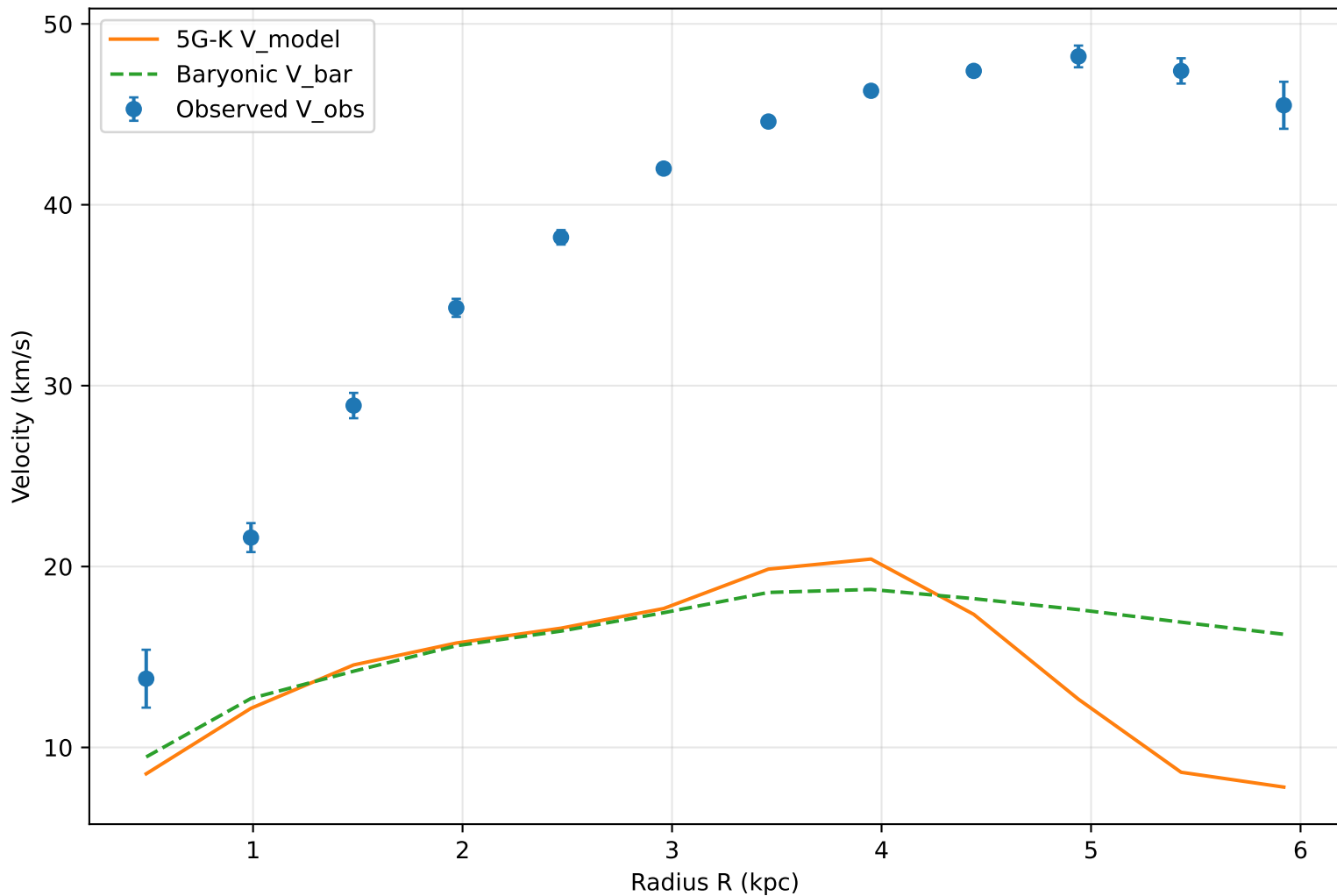
5G-K Variational Scheduler: DDO154
