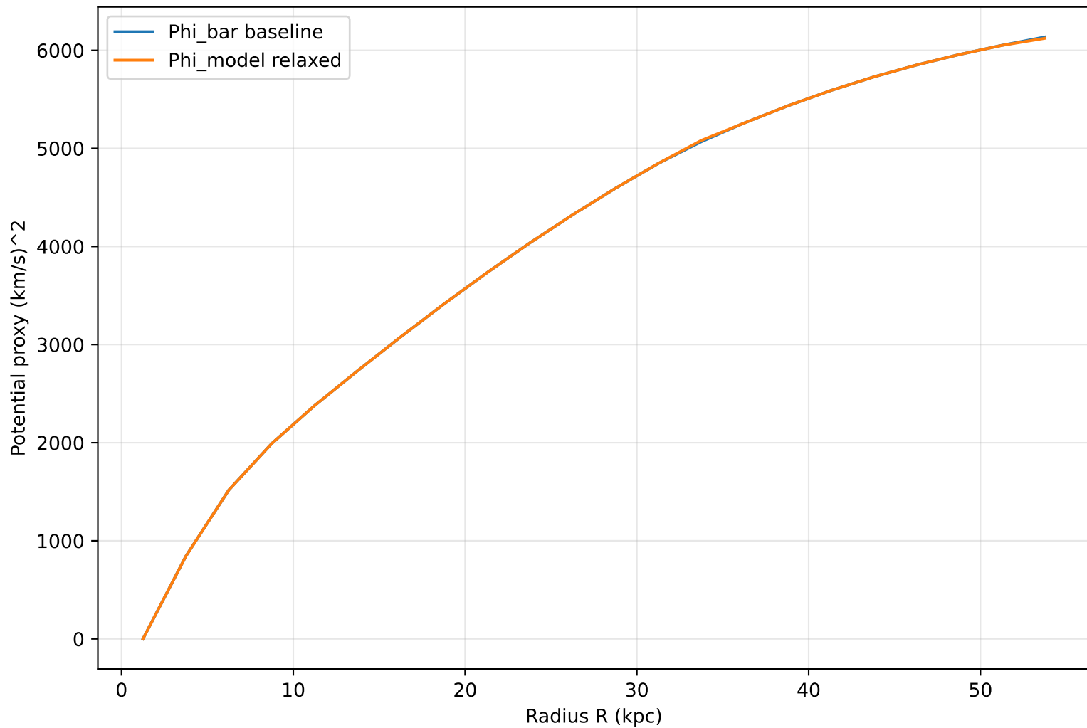
Potential field relaxation: UGC00128
