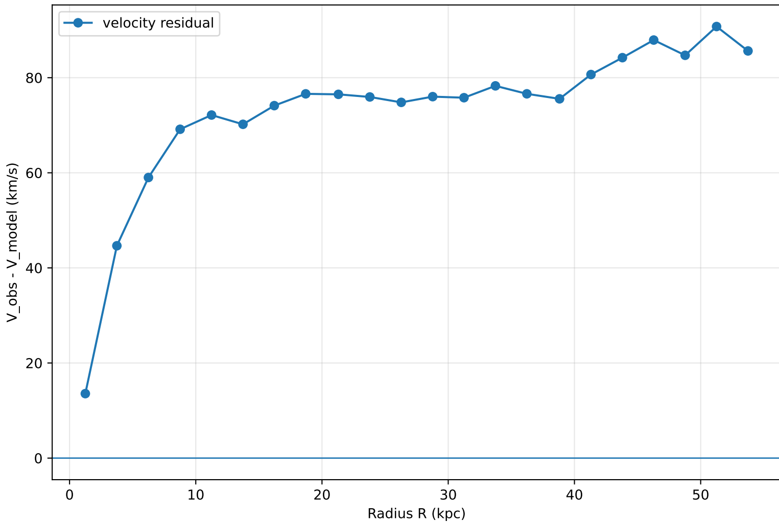
5G-K residual: UGC00128
