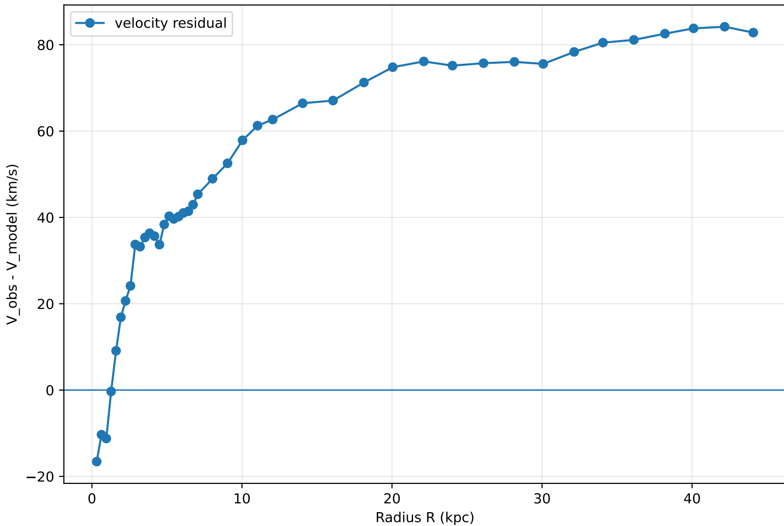
5G-K residual: NGC3198
