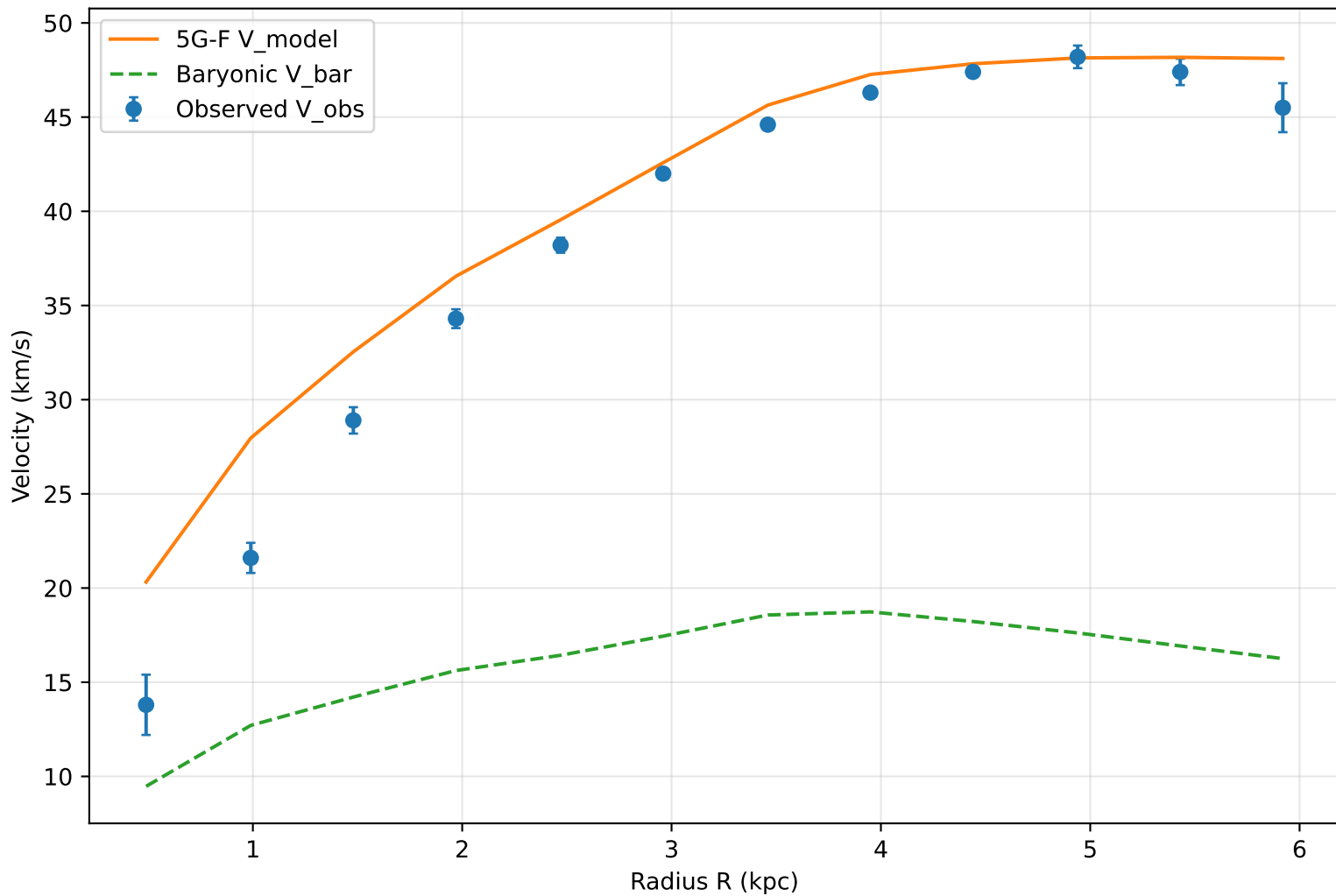
5G-F Nonlocal Kernel: DDO154
