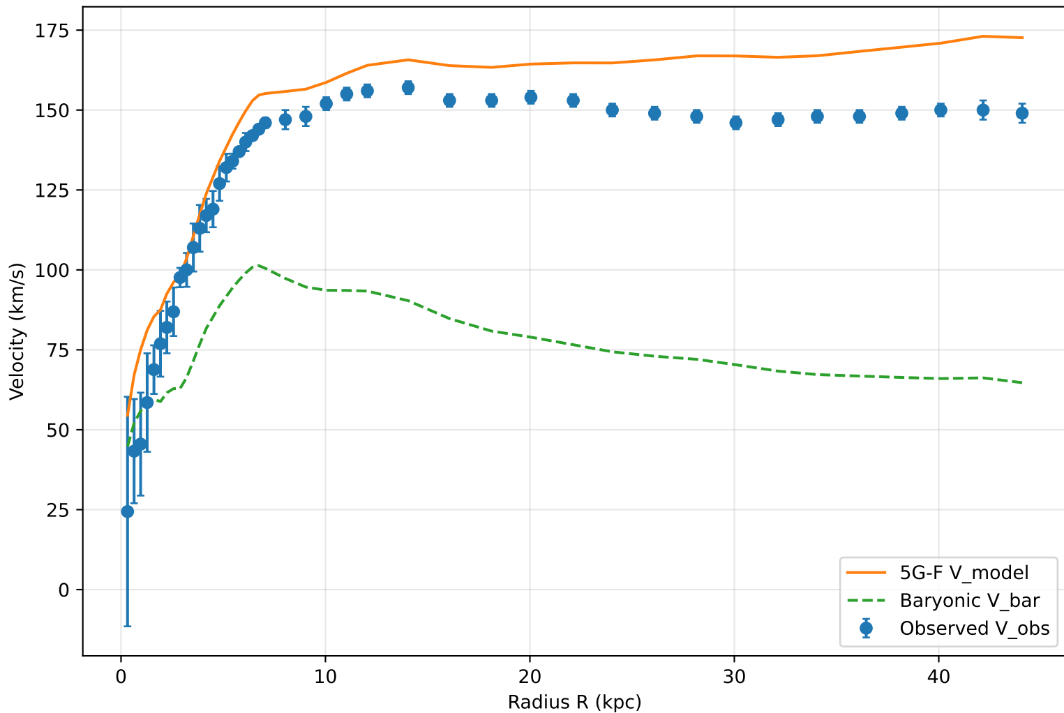
5G-F Nonlocal Kernel: NGC3198
