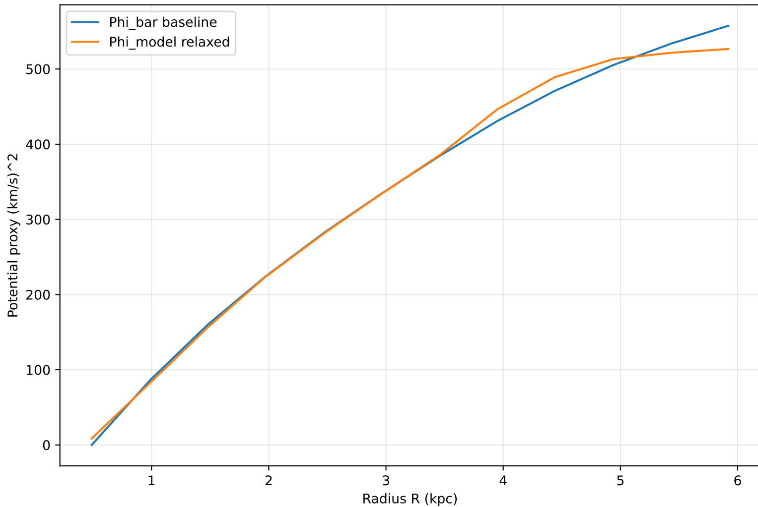
Potential field relaxation: DDO154
