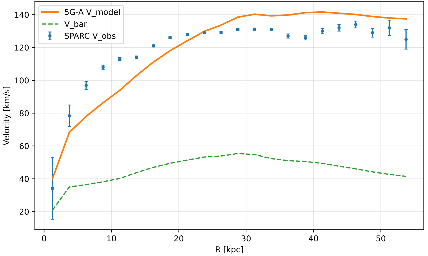
Toy Model 5G-A — UGC00128 (predeclared sample galaxy)
