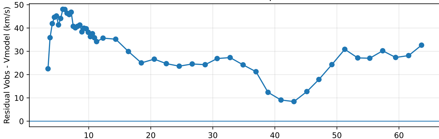
5G-F Residual and Nonlocal Response: NGC2841
